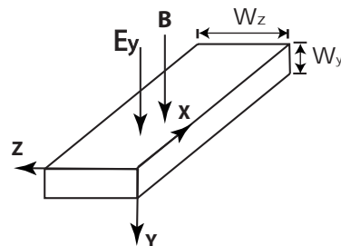
FIG. 1. Geometry of the quantum wire. For our numerical calculations, we assumed that the width of the wire along the z direction is 100 nm and the thickness of the wire along the y direction is much smaller so that only the lowest transverse subband in the y direction is occupied. The y -directed electric field E_y induces a Rashba spin-orbit interaction in the channel, and B is an external magnetic field, also applied in the y direction.
