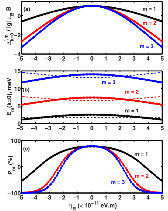
FIG. 8. (Color online) (a) The zero- k spin splitting energy ( \Delta'_{k=0} ) in the lowest three subbands as a function of the Rashba interaction strength \eta_R . This quantity decreases and eventually flips sign as the magnitude of the Rashba interaction strength ( |\eta_R| ) is increased. The Dresselhaus constant \gamma_D has a fixed value of 0.5 \times 10^{-11} eV m, and the external magnetic flux density B = 1 T. This figure also shows that \Delta'_{k=0} is an even function of \eta_R . (b) Variation of the energy at the bottom of each spin-split level in the lowest three subbands with \eta_R . The two spin levels are denoted by solid and broken lines. In each subband, the spin levels cross at some value of |\eta_R| , which gives rise to the zero crossings in the top panel. (c) The equilibrium spin polarizations of carriers in the lowest three subbands as functions of \eta_R at temperature T = 5 K.
