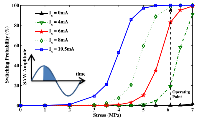
FIG. 2. Probability of a magnet switching at room temperature in 5 ns (half-period of the 100 MHz SAW) as a function of the peak stress generated by the SAW. The various curves are for different spin-polarized currents. Note that the probability of switching in the absence of spin polarized current remains zero up to a peak stress of 6.1 MPa. The spin-polarized current is turned on for the latter half of the appropriate half-cycle of the SAW (2.5 ns) as shown in the inset (shaded region) to write the bit.
