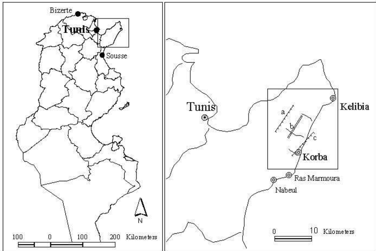
Figure 1: Location map of the Korba coastal plain in northeastern Tunisia on the Mediterranean Sea (left) and enlargement showing the population centers and the main hydrographic (ephemeral streams) and geologic (anticline and syncline) features (right).
