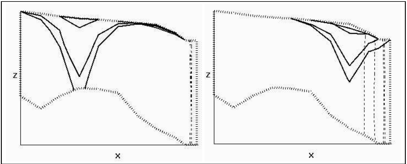
Figure 5: Simulation results for two experiments plotted as vertical cross sections perpendicular to the coast and passing through the town of Korba, comparing the groundwater drawdown and seawater intrusion from inland (left) and coastal (right) pumping regimes and illustrating the interaction between the unsaturated zone and the saltwater–freshwater interface. The two plots show water table levels and 0.5 normalized salinity isolines at times 1, 6, 25, and 35 years in response to pumping from a single well at a rate that increases linearly over the 35-year simulation period from 0 to 0.91 \times 10^6 \text{ m}^3/\text{yr} .
