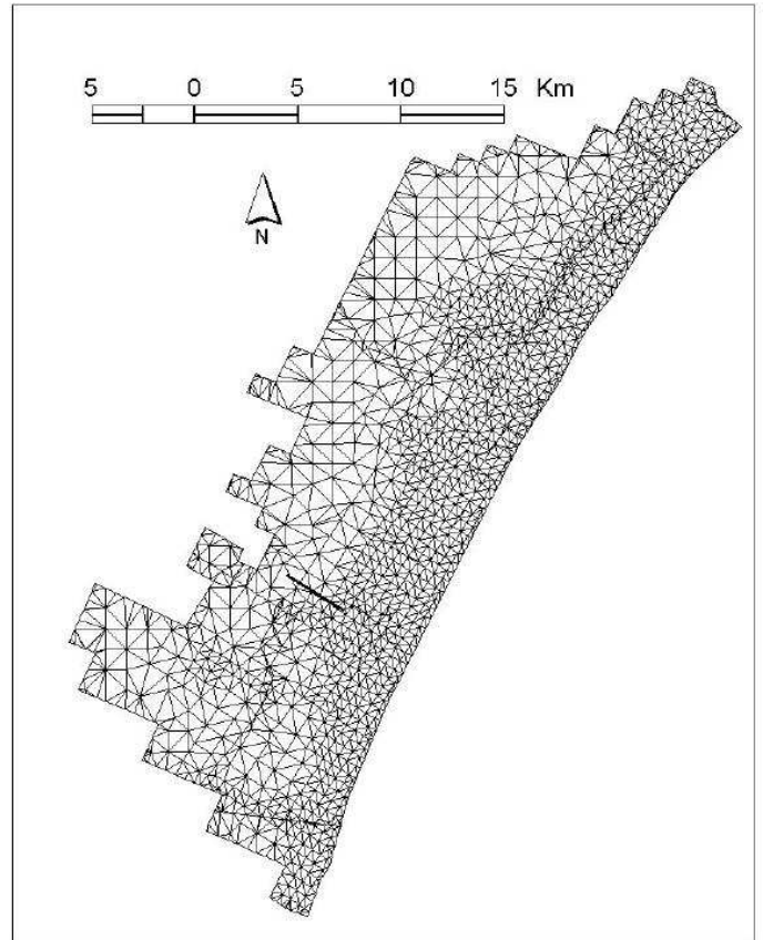
Figure 4: Surface discretization of the modeled area into 2917 triangles, with the smallest elements near the coast and around important pumping well clusters. This nonuniform surface grid was replicated vertically for 6 layers of varying thickness (thinnest layers near the surface) to yield a three-dimensional mesh containing 52506 tetrahedral elements and 11501 nodes.
