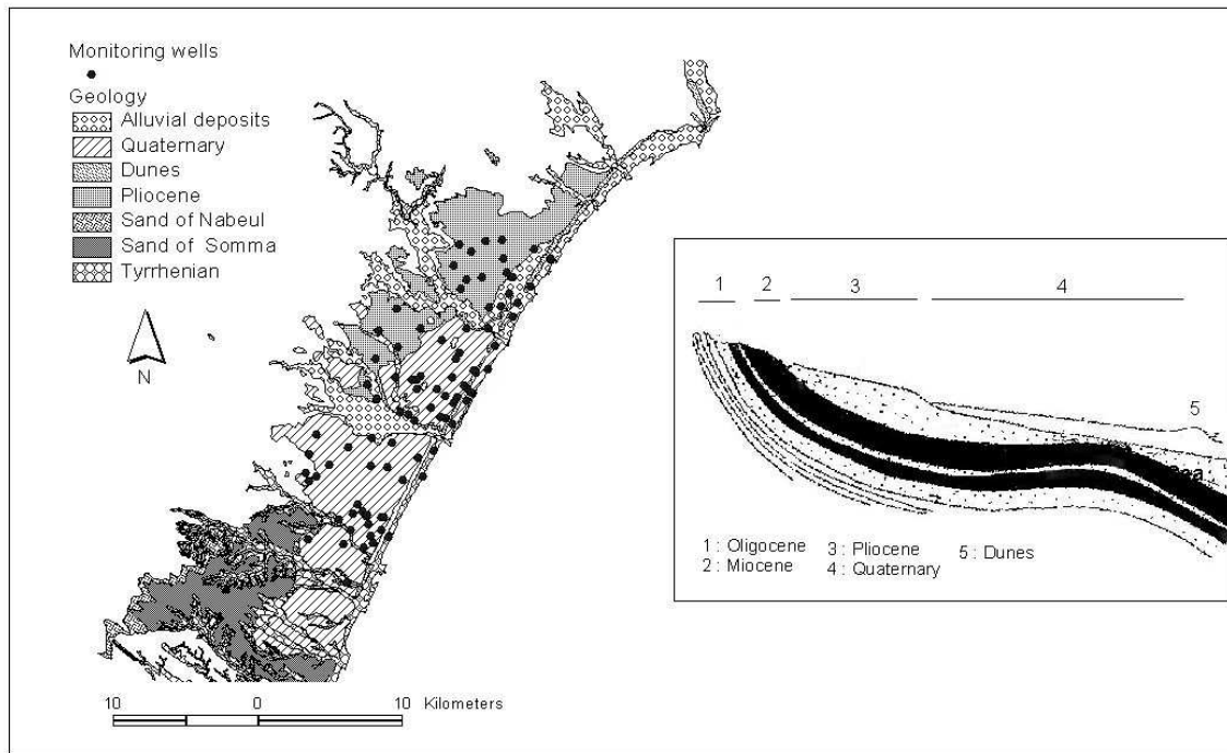
Figure 2: Simplified geologic map of the Korba study area derived by aggregation of surface geologic features into dominant units (left); vertical geologic cross section perpendicular to the coast and passing roughly midway through the aquifer showing the anticline, syncline, and dune formations that determine the shape and varying thickness of the Quaternary–Pliocene unconfined aquifer, along with underlying formations (right).
