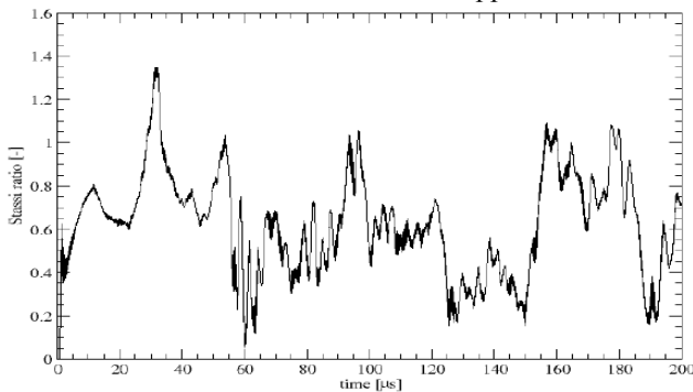
Figure 6. 200 \mu s evolution of stress ratio for block 15.
