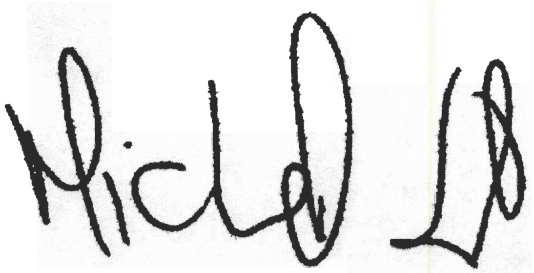
Figure 3.1 : Image originale.
