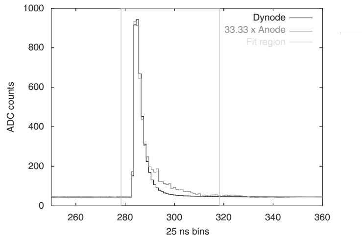
Fig. 6. Example of the D/A fit to a resistively-divided pulse with the preproduction front end electronics. The pulse generator had an intrinsic D/A of 33.9, and the D/A fit method gave a D/A of 33.3, within 2%. The excess in the anode seen near 300 time bins is \sim 1 ch, which is the noise level of the preproduction electronics. The fit clearly determines the proper D/A even in the presence of < 1 ch noise.
