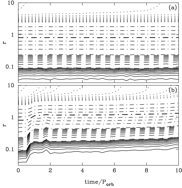
Fig. 5. Lagrangian radii for the cluster mass in the simulation with our centering routine (a), and the live particle method (b). The solid lines correspond to 0.1%, ..., 0.9%, the dashed lines to 1%, ..., 9%, the dashed and dotted lines to 10%, ..., 50% (thick line), ..., 90%, and the dotted lines to 91%, ..., 99% of the mass.
