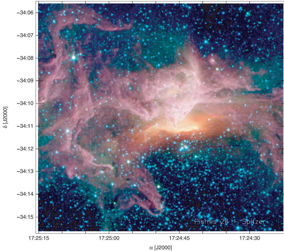
Figure 9. Enlargement of the G353.2+0.9 region as shown by the emission in the IRAC bands: 3.6 \mu\text{m} is in blue, 4.5 \mu\text{m} in green and 8 \mu\text{m} in red.
