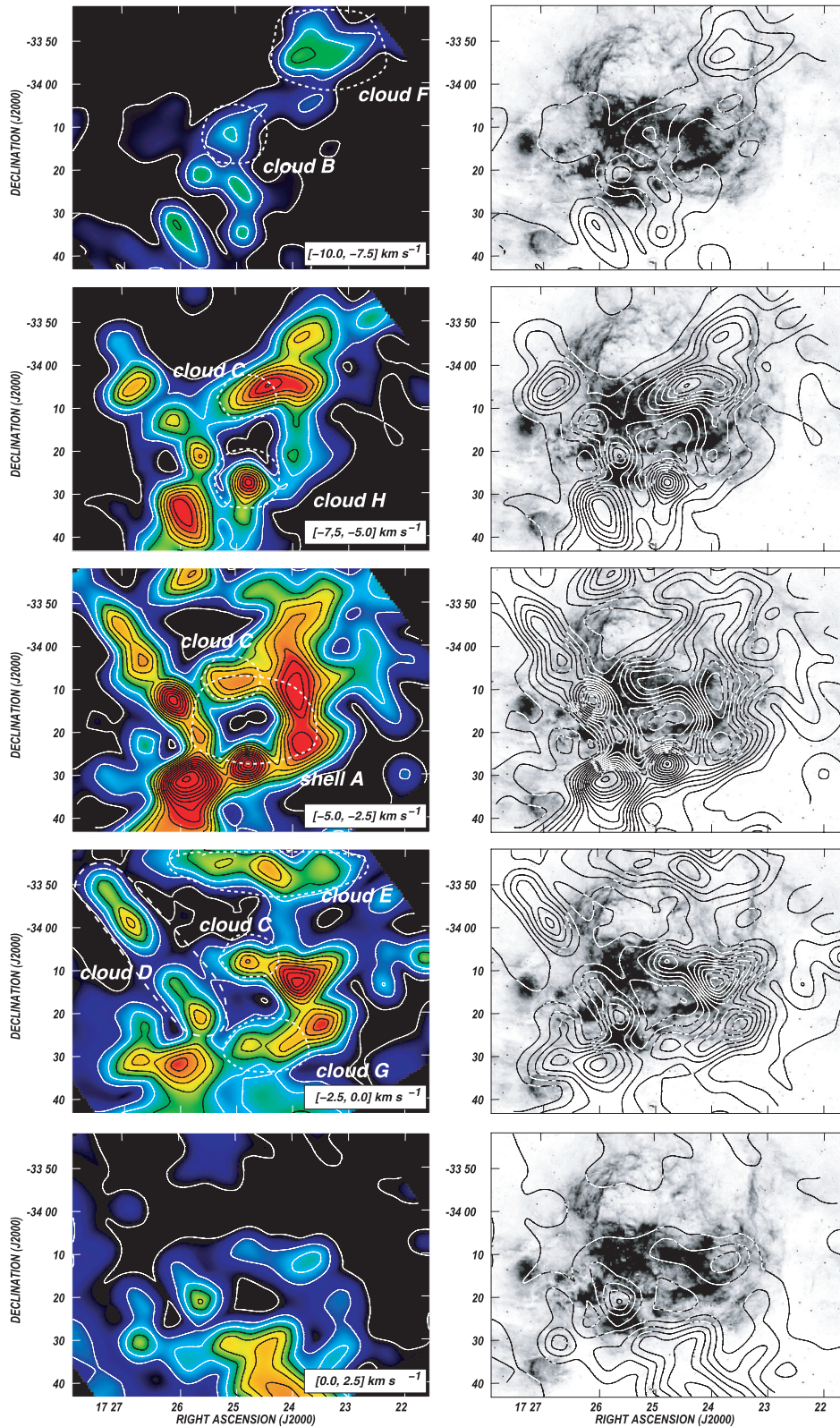
Figure 8. Left panels: ^{12}\text{CO}(1-0) emission distribution within the velocity interval [-10.0, +2.5] \text{ km s}^{-1} in steps of 2.5 \text{ km s}^{-1} . The velocity interval is indicated in the bottom-right corner of each image. Intensities are expressed as main beam brightness temperature averaged over each velocity interval. Contour levels start at 0.7 \text{ K} ( \equiv 12.5\sigma ), increasing in steps of 1.75 \text{ K} . Colour scale goes from 0.7 (dark blue) to 10.5 \text{ K} (red). The angular resolution of the CO data is 2.6 \text{ arcmin} . Shell A, as well as clouds B, D, E, F, G and H are indicated only in one map, although they span a larger velocity interval. Right panels: overlay of the same CO contours of the left-hand panels and the \text{H}\alpha image.
