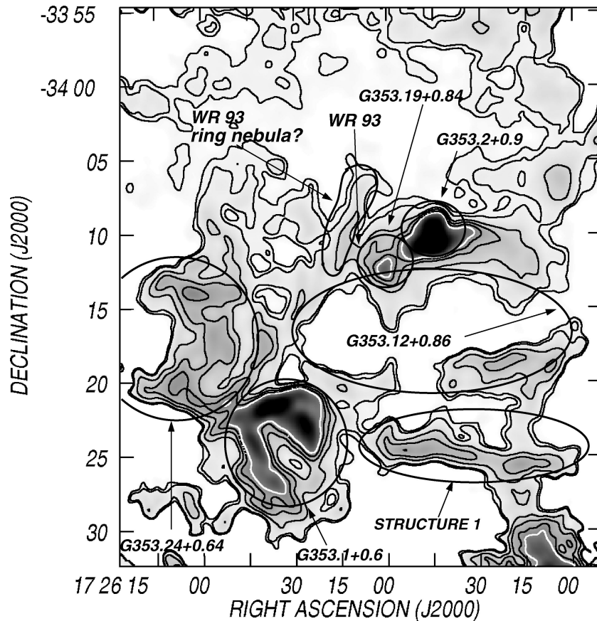
Figure 5. VLA image at 1.46 GHz of the NGC 6357 complex. Grey-scale ranges from -0.01 to 6.6 \text{ Jy beam}^{-1} . Contours correspond to 0.05, 0.10, 0.30, 0.50, 0.75 and 1.0 \text{ Jy beam}^{-1} . Identified structures and the position of WR 93 are indicated. The synthesized beam is 43.9 \times 34.3 \text{ arcsec}^2 at a position angle of +41^\circ . The rms noise in the central part of the image is 20 \text{ mJy beam}^{-1} .
