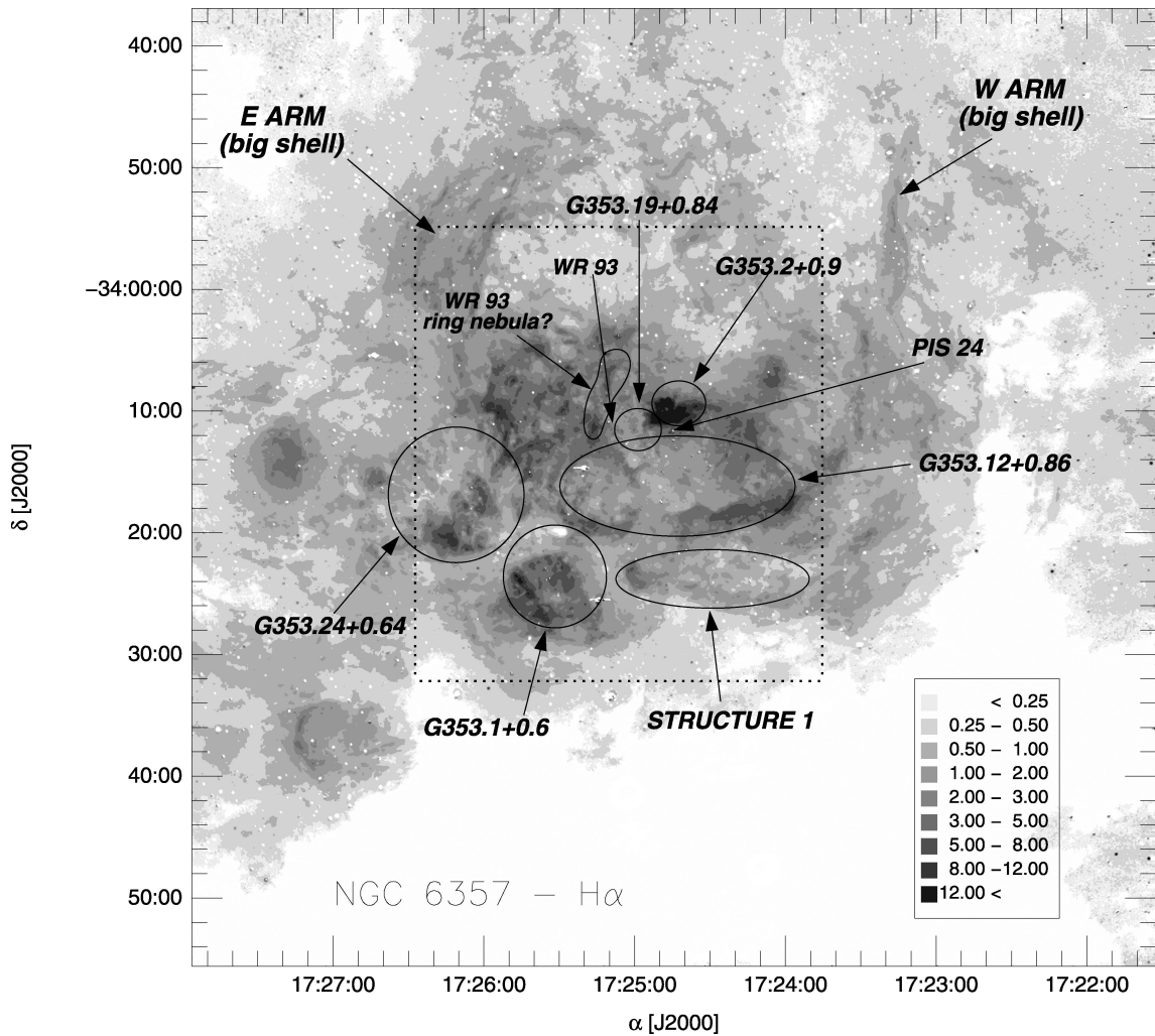
Figure 2. Continuum-subtracted H\alpha image of NGC 6357 obtained at CTIO. Different structures in the ionized complex are indicated to facilitate their identification in Fig. 1. The grey-scale values are in the unit of 10^{-14} erg \text{cm}^{-2} \text{s}^{-1} \text{pix}^{-1} . The dotted line delineates the region observed at 1.46 GHz.
