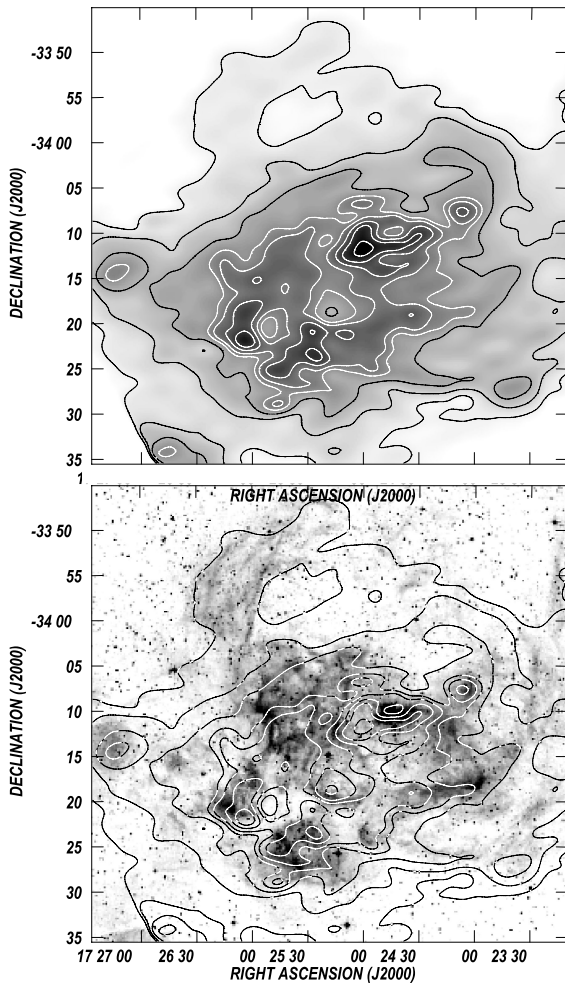
Figure 6. Top panel: dust colour temperature T_c estimated from the IRAS images at 60 and 100 \mu\text{m} . Contours range from 33 to 54 K in steps of 3 K. The grey-scale ranges from 33 to 54 K (areas in black correspond to the highest temperatures). The image was smoothed to 2 arcmin. Bottom panel: overlay of the dust colour temperature (contours) and the H\alpha emission (grey-scale).
