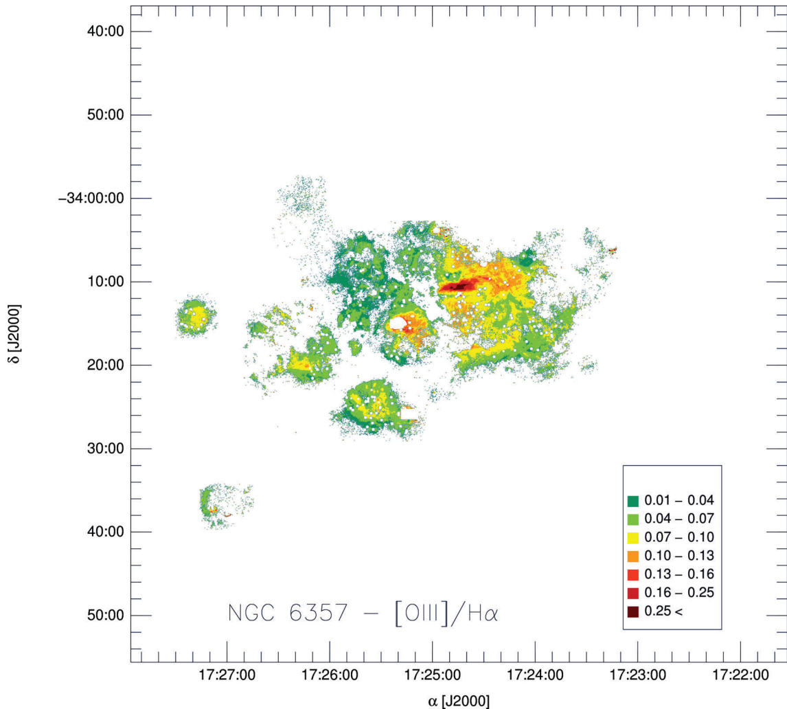
Figure 4. [\text{O III}]/\text{H}\alpha line ratio. Continuum was subtracted from the individual images. The colour scale is indicated in the lower-right corner of the image. White areas correspond to regions below the cut-off value.
