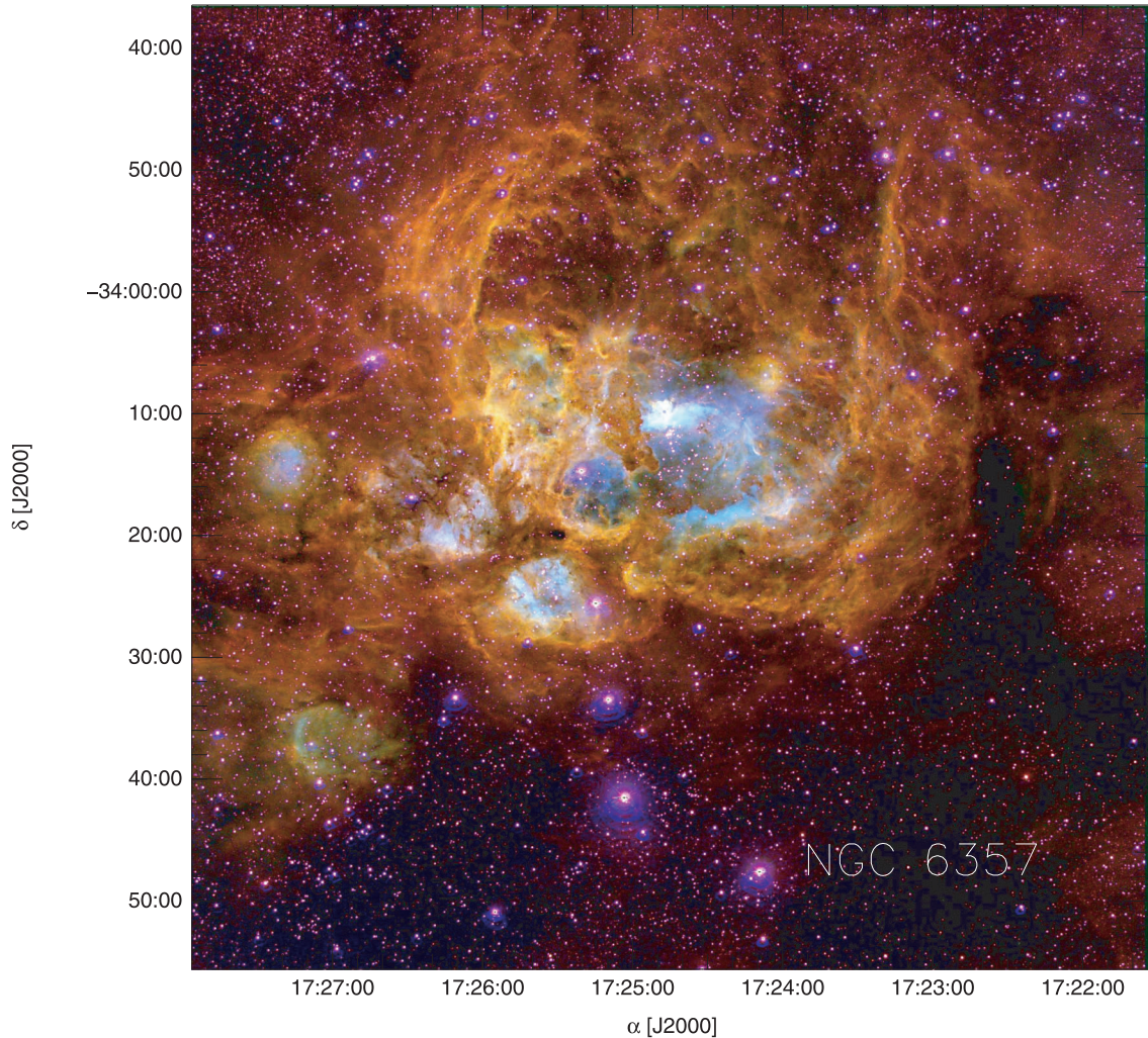
Figure 1. Colour composite image of NGC 6357. Red, green and blue show emission from [S II] 6716–31 Å, H \alpha and [O III] 5007 Å, respectively. These images were obtained with the Curtis–Schmidt camera at CTIO during 1999.
