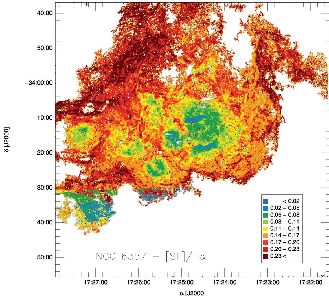
Figure 3. [\text{S II}]/\text{H}\alpha line ratio using the images obtained at CTIO. Continuum was subtracted from the individual images. The colour scale is indicated in the lower-right corner of the image. White areas correspond to regions below the cut-off value.
