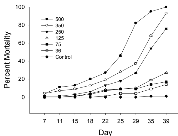
Figure 6. Mortality (%) (mean ± SE) of S. oryzae adults fed ad libitum with flour disks treated with 36, 75, 125, 250, 350 and 500 ppm of NSA after 39 days in the intake toxicity bioassay.
