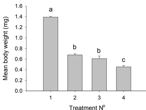
Figure 7. Mean individual body weight of S. oryzae adult exposed to different dehydration treatments after 72 hours at 27 ± 1 °C and 75% RH. 1: control group fed in untreated wheat ad libitum ; 2: insects slay with chloroform and incubated; 3: live insects exposed to wheat treated with NSA 500 ppm; 4: dead insects incubated at 60 °C. Bars with different letters are statistically different (ANOVA: P < 0.0001).
