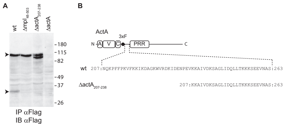
FIG 4 Mapping of an Mpl-dependent processing site in ActA. (A) Western blot of ActA 3×F immunoprecipitated (IP) from cell lysates infected with L. monocytogenes wild-type, \Delta mpl_{48-503} , \Delta actA_{207-238} , or \Delta actA strains. Arrowheads indicate ActA peptides of 90 and 30 kDa. Apparent molecular weights (in thousands) in the protein ladder are indicated on the right. IB, immunoblot. (B) Schematic representation of 3×Flag-ActA and in-frame deletion of ActA residues 207 to 238. Numbers indicate the first and last residues.
