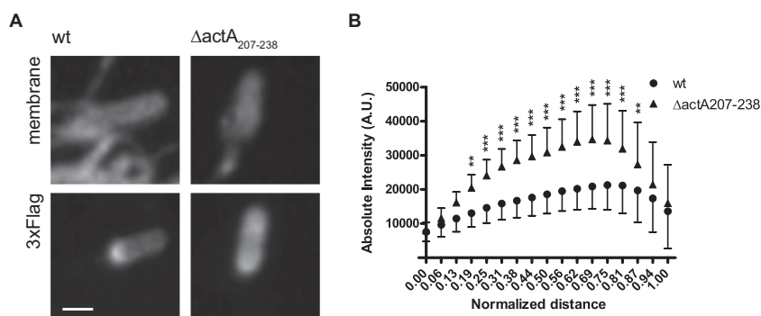
FIG 5 Distribution of ActA on the surface of wild-type and \Delta actA_{207-238} mutant bacteria forming protrusions. (A) Representative images showing the distribution of 3×Flag-ActA on the surface of bacteria in protrusions. Top panels, plasma membrane. Bottom panels, FLAG staining. Bar, 1 \mu m. (B) Quantification of ActA distribution on the bacterial surface. The absolute intensity of the FLAG signal is represented against the normalized distance from the front pole. Data are represented as means and standard deviations and were analyzed by two-way ANOVA using PRISM 5 (GraphPad Software). ***, P < 0.001 ; **, P < 0.01 ; *, P < 0.05 .
