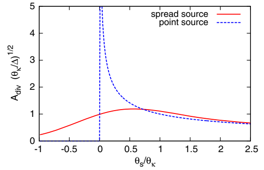
FIG. 8. Average magnification multiplied by \sqrt{\theta_{\kappa}/\Delta} , as a function of the normalized angular distance from the source to the fold.
