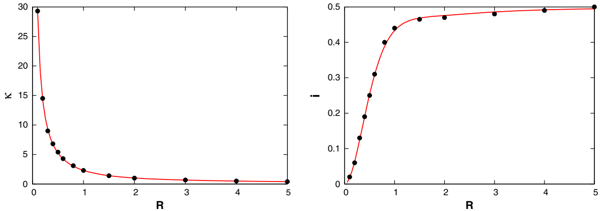
FIG. 3. Parameters \kappa (left) and i (right) as a function of the normalized source distance.
