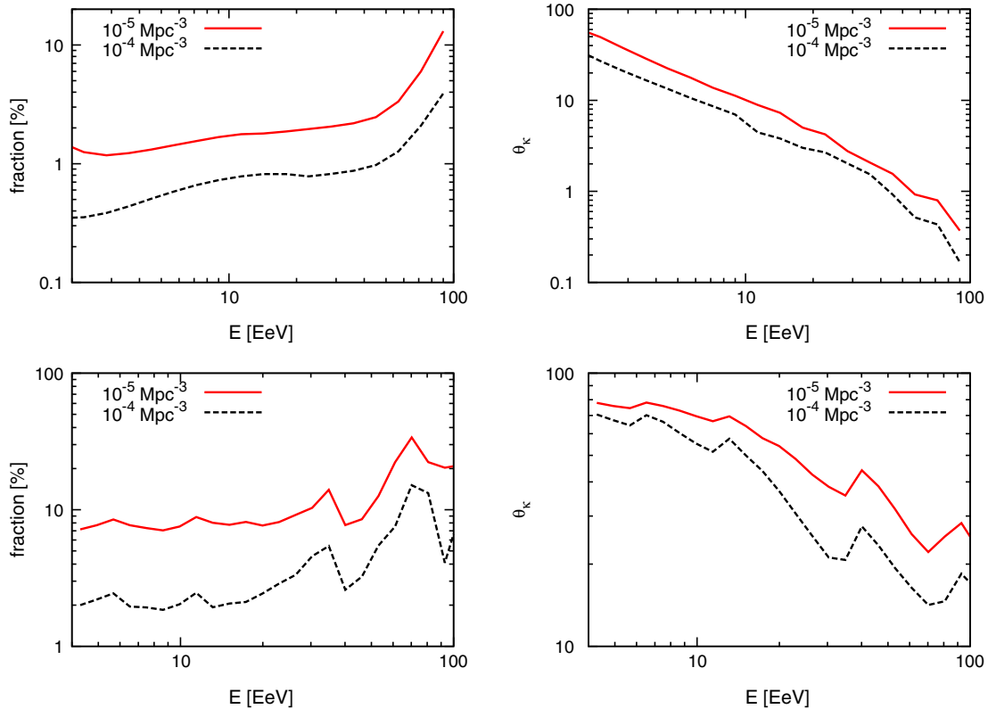
FIG. 7. Left: fraction of the total flux that is expected to arrive from the closest source for two values of the source density. Right: angular spread (in degrees) of the distribution of the cosmic rays coming from the closest source. We assumed equal luminosity sources at distances equal to the corresponding expected mean values. The top panels are for proton sources while the lower ones are for nuclei adopting fractions of p , He, N, Si, and Fe nuclei as described in the text, with a maximum energy of 6Z EeV.
