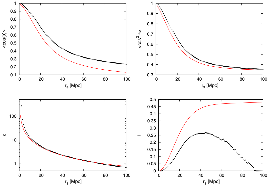
FIG. 6. Values of \langle \cos \theta \rangle , \langle \cos^2 \theta \rangle , \kappa , and i as a function of r_s for a proton source and for final energies of 2.7 EeV. Dots include the effects of energy losses while the lines neglect them.
