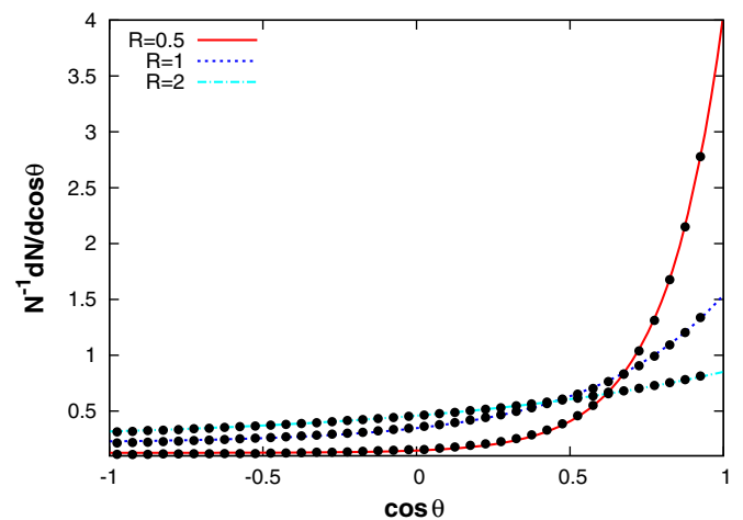
FIG. 1. Distribution of CR arrival directions as a function of \cos \theta for three values of the normalized source distance R \equiv r_s/l_D = cr_s/3D = 0.5, 1 , and 2 . The lines indicate the fits using the expression in Eq. (4).
