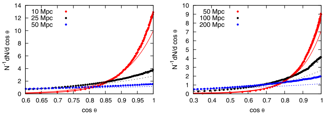
FIG. 4. Distribution of arrival directions for three values of the source distance but including energy losses. The left panel is for E = 3E_c(0) = 2.7 EeV and the right one for E = 6E_c(0) = 5.4 EeV [using B_{\text{rms}}(0) = 1 nG and l_c(0) = 1 Mpc]. Note that l_D(0) = 39 Mpc for E = 3E_c(0) , while l_D(0) = 150 Mpc for E = 6E_c(0) . The thin lines correspond to the analytic expressions that would be obtained without energy losses while the fits including the energy losses overlap with the simulated points.
