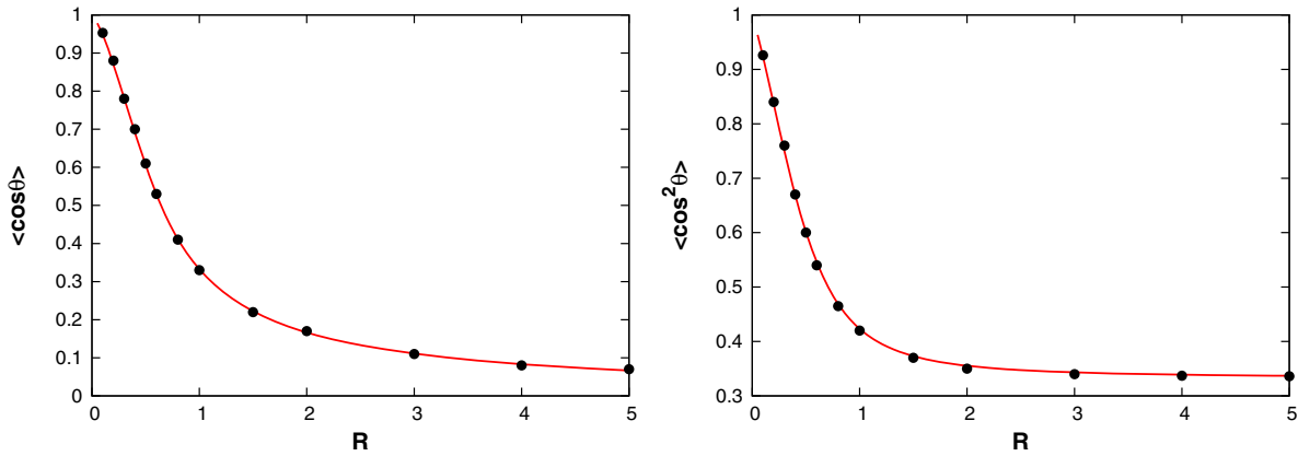
FIG. 2. Average \cos \theta (left) and \cos^2 \theta (right) as a function of the normalized source distance R \equiv r_s/l_D = cr_s/3D .
