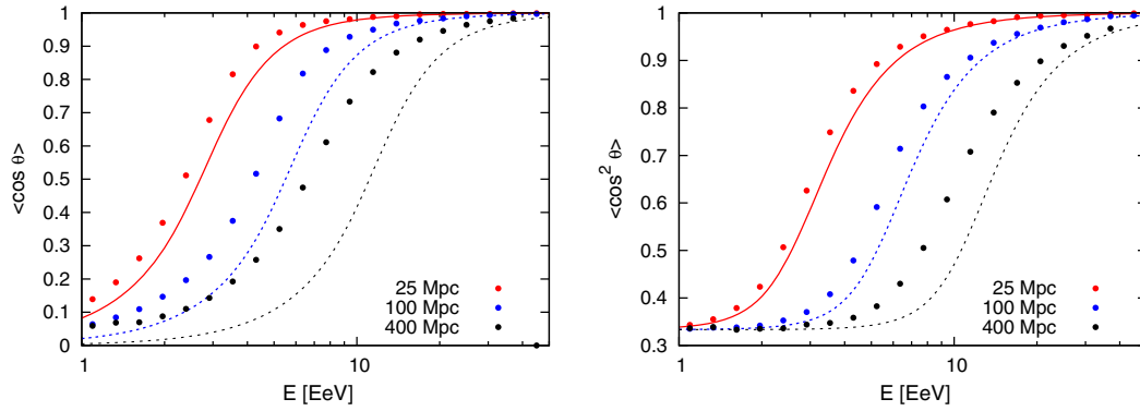
FIG. 5. Values of \langle \cos \theta \rangle and \langle \cos^2 \theta \rangle as a function of the arrival energy E for three values of the source distance. Points include energy losses while the lines are the corresponding results in the absence of losses.
