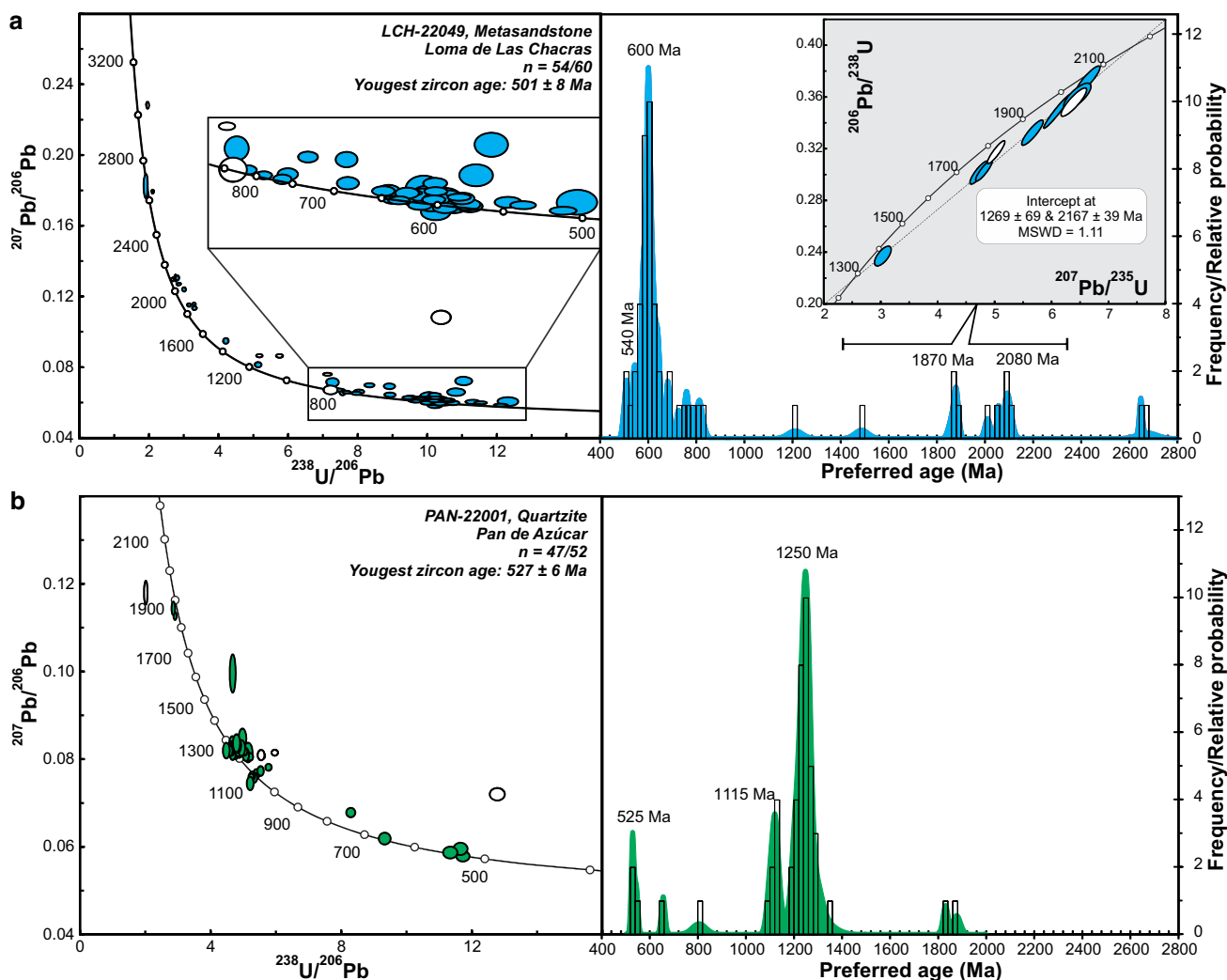
Fig. 8 Tera–Wasserburg and probability density plots from sample LCH-22049 (metasandstone; Loma de Las Chacras) (a) and sample PAN-22001 (quartzite; Sierra de Pan de Azúcar) (b)
