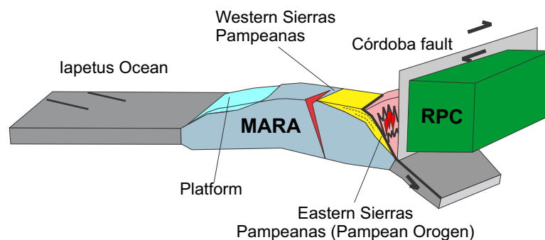
Fig. 3 Geotectonic evolution of southern SW Gondwana between ca. 620 Ma and the end of the Pampean orogeny at ca. 520 Ma preceding eastward extension of the sedimentary platform. Modified after Casquet et al. (2012a). RPC = Río de la Plata craton (ca. 2.02–2.25 Ga)
