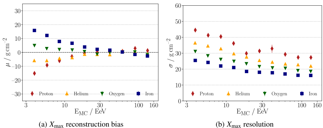
Figure 4. EPOS-LHC simulation study: energy-dependent (a) bias and (b) resolution of the X_{\max} reconstruction evaluated on EPOS-LHC showers with the deep neural network also trained using EPOS-LHC showers. Different colors indicate different primaries.
