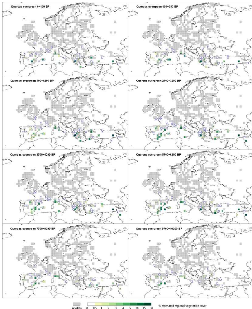
Figure D3. Grid-based REVEALS estimates of evergreen Quercus cover for eight Holocene time windows. Percentage cover in 0.5% intervals between 0% and 1%, 1% intervals between 1% and 5%, 5% intervals between 5% and 15%, and 15% intervals between 15% and 30%. See caption of Fig. A1 for more explanations. Intervals represented by increasingly darker shades of green from 1%–2%. Grey grid cells have no data (pollen) for Calluna vulgaris in the mapped time window. The circles represent the coefficient of variation (CV; the standard error divided by the REVEALS estimate). When SE \geq REVEALS estimate, the circle fills the entire grid cell, and the REVEALS estimate is not different from zero. This occurs mainly where REVEALS estimates are low.
