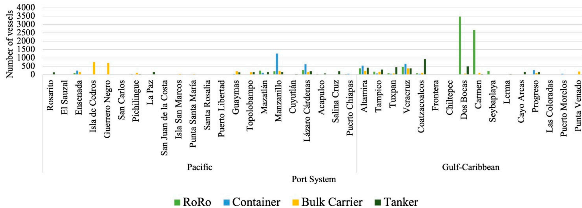
Figure 6. Arrivals by type of vessel at each Mexican port during 2020.
