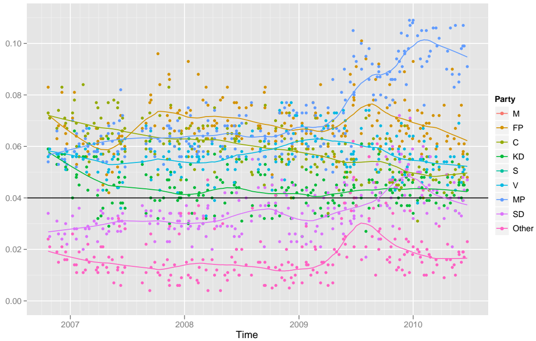
Figure 3: Close-up of the smoothed Swedish opinion poll series with q = 40 with original observations. The solid black line represents the 4% election threshold for winning seats in the Swedish parliament.
