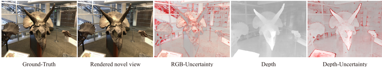
Figure 1. Illustration of the results obtained by Stochastic Neural Radiance Fields (S-NeRF). Our method is a probabilistic generalization of the original NeRF, which is able to not only address tasks such as novel-view generation (Rendered novel view) or depth-map estimation (Depth), but also quantify the uncertainty (red color) associated with the model outputs. This is specially important in domains such as robotics, where this information is necessary to evaluate the risk associated with decisions based on the model estimations.
