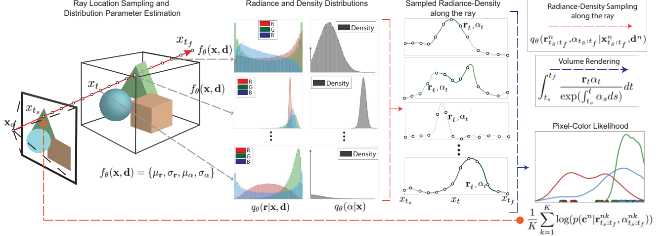
Figure 2. Illustration of the pipeline used by S-NeRF to compute the log-likelihood of the pixel color in a given view. From left to right: (i) For each coordinate \mathbf{x} along a camera ray with viewing direction \mathbf{d} , a neural network predicts the parameters of the radiance and density distributions. (ii) For each spatial-location, we sample a set of radiance-density pairs from the previous distributions. (iii) This generates a set of different radiance-density trajectories along the ray obtained from a distribution of radiance fields. (iiii) The volume rendering equations are used to estimate the RGB values for each trajectory and compute the log-likelihood for a given pixel color. During inference, the mean and variance of these samples are used as the model prediction and to quantify its associated uncertainty.
