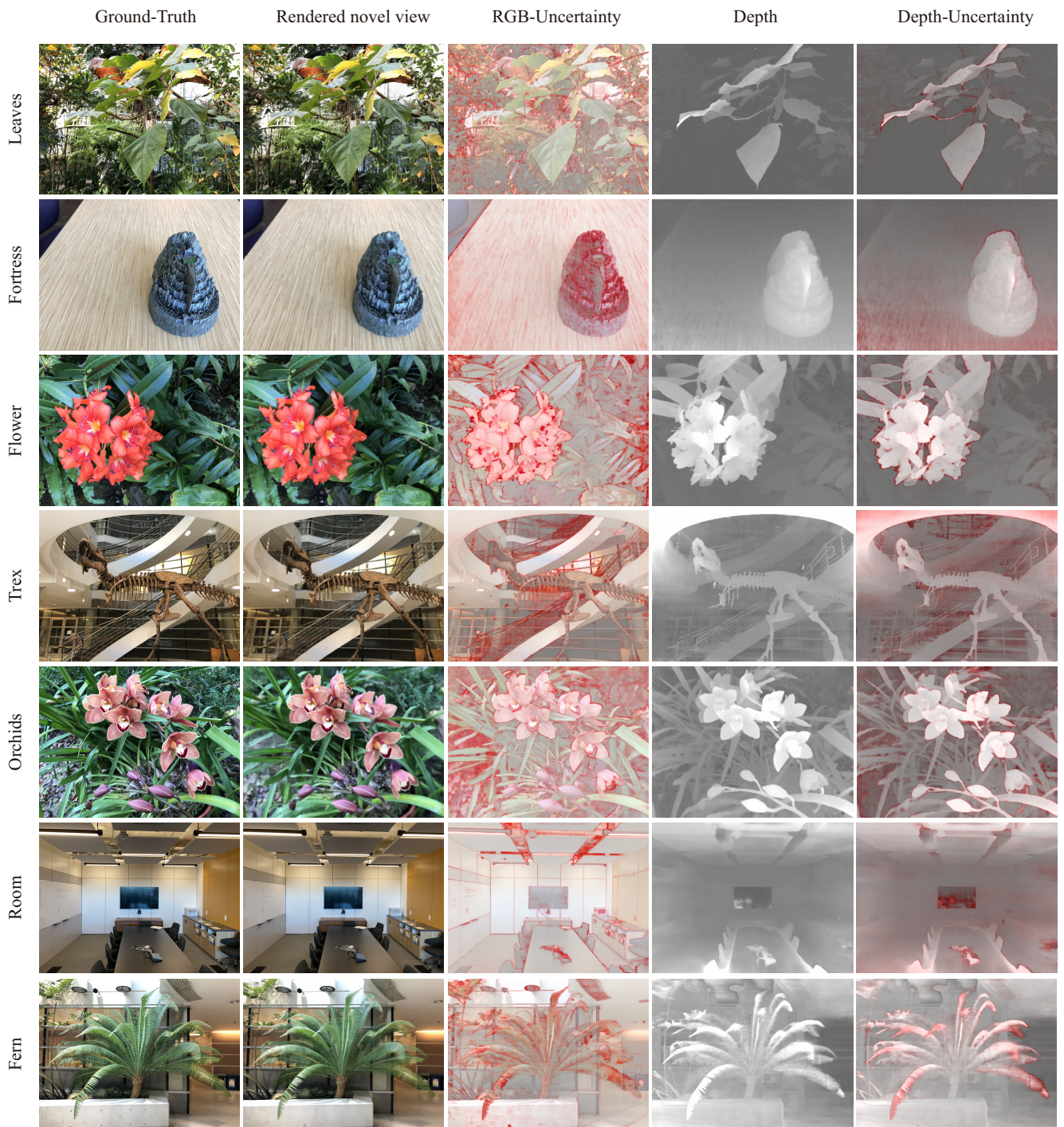
Figure 6. Additional qualitative results obtained by our S-NeRF.
