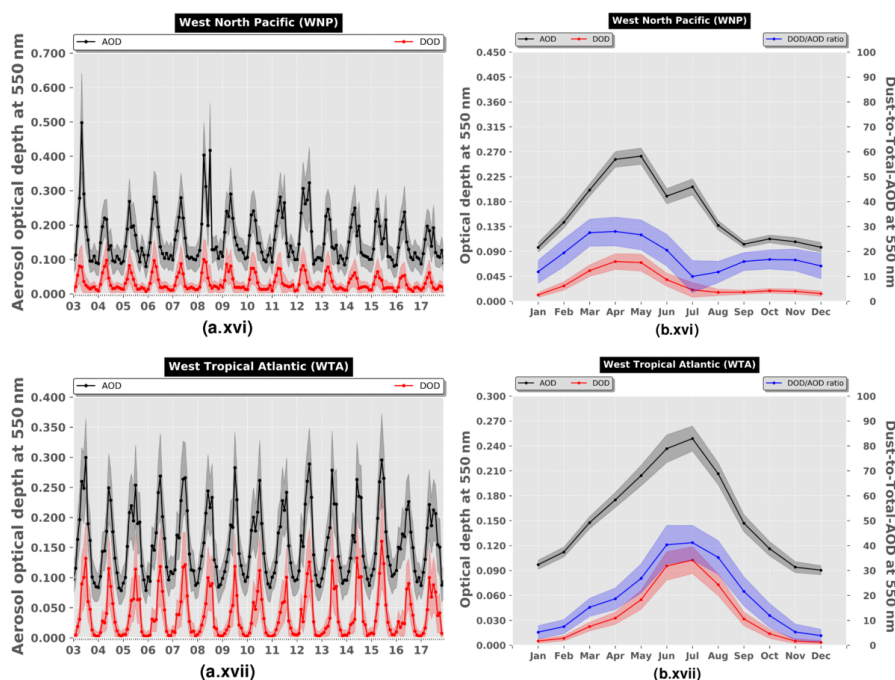
Figure 11. Interannual (a) and intra-annual (b) variability, representative for the period 2003–2017, of monthly MODIS AOD_{550\text{ nm}} (black curve) and DOD_{550\text{ nm}} (red curve) regionally averaged for (i) Bodélé Depression (BOD), (ii) Gobi Desert (GOB), (iii) Central Asia (CAS), (iv) north Middle East (NME), (v) southwest United States (SUS), (vi) Taklamakan Desert (TAK), (vii) Thar Desert (THA), (viii) Western Sahara (WSA), (ix) East Asia (EAS), (x) east North Pacific (ENP), (xi) east tropical Atlantic (ETA), (xii) Gulf of Guinea (GOG), (xiii) Mediterranean (MED), (xiv) south Middle East (SME), (xv) sub-Sahel (SSA), (xvi) west North Pacific (WNP) and (xvii) west tropical Atlantic (WTA). The shaded areas in the inter- and intra-annual plots correspond to the total uncertainty. The blue curves in the intra-annual plots represent the percentage contribution of dust optical depth (DOD) to the aerosol optical depth (AOD).
