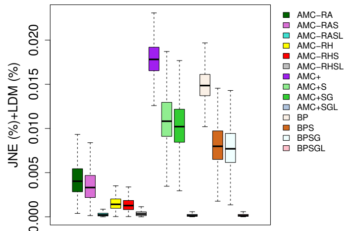
Fig. 6. Results for JNE + LDM(\%) - 80% LO-criticality Utilization: Non-Harmonic Periods.
