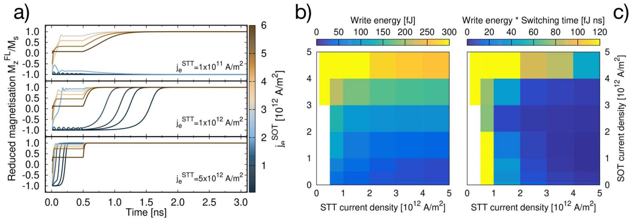
Figure 4. (a) Time evolution of the reduced z-component of the magnetisation as a function of j_e^{\text{SOT}} for j_e^{\text{STT}} = 1 \times 10^{11}, 1 \times 10^{12} and 5 \times 10^{12} \text{ A/m}^2 . In this case A_F = A_D and the diameter is 20 nm. (b) Write energy and c) write energy \times total switching time as a function of j_e^{\text{STT}} and j_e^{\text{SOT}} for A_F = A_D and diameter of 20 nm. The palette represents the energy in (b) and energy \times switching time in (c), and ranges from blue (low) to yellow (high). White regions correspond to combinations of j_e^{\text{STT}} and j_e^{\text{SOT}} that yield no switching.
