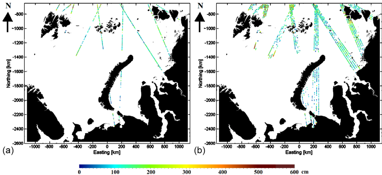
Figure 1. CryoSat-2 sea ice thickness measurements during 1 d (a) and 1 week (b) before 21 February 2017.
