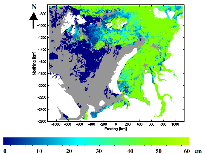
Figure 13. MODIS SIT collage based on 2 weeks of MODIS daily SIT charts before 21 February 2017. The areas without data are indicated by the grey colour, and all the ice thicker than 50 cm is indicated by the green colour, corresponding to 60 cm in the colour map.
