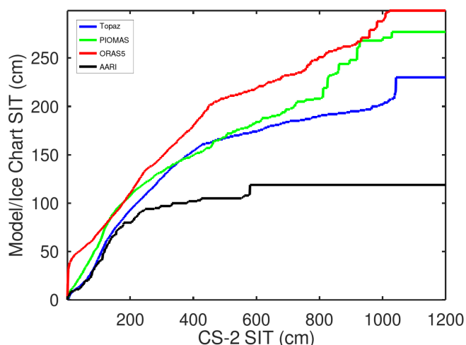
Figure 8. The correspondence of the CryoSat-2 SIT to AARI ice chart SIT and modelled SIT from the three models studied based on histogram matching.
