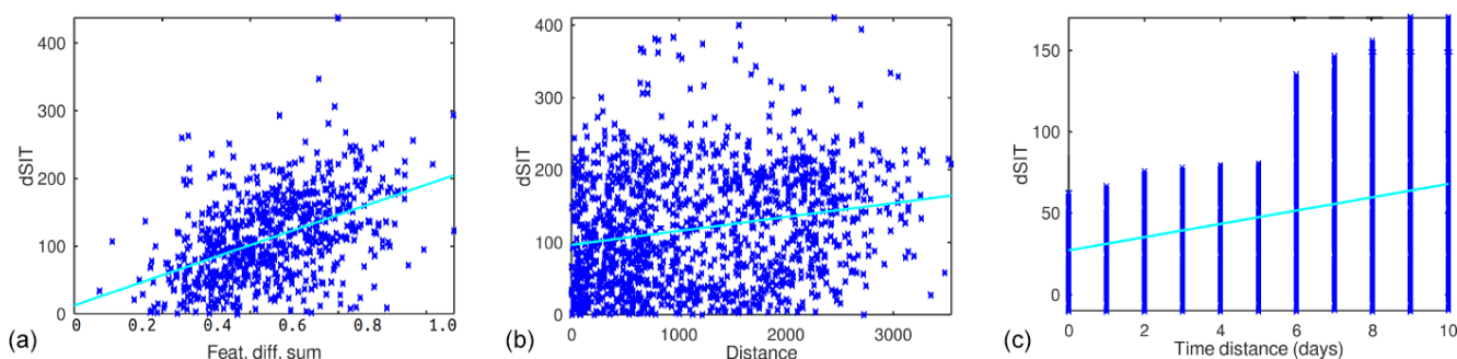
Figure 7. (a) Dependence of the SIT difference on the pairwise SAR segment texture difference, (b) dependence of the SIT difference on the pairwise SAR segment distance and (c) dependence of the SIT difference on the pairwise SAR segment time difference. The cyan lines in the figures represent the linear least-squares regression.
