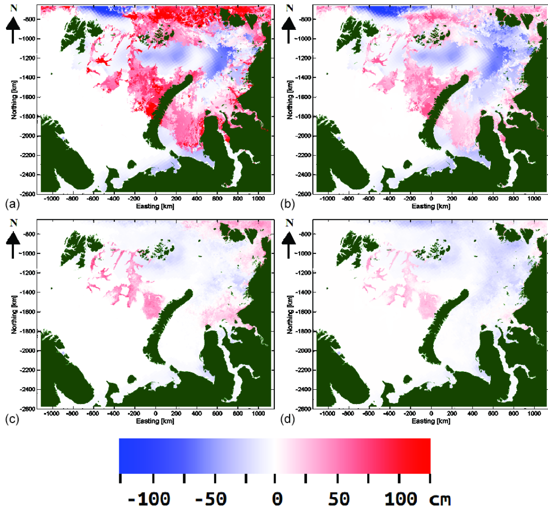
Figure 11. (a) Difference of the proposed (unmapped) SIT and CS2SMOS SIT for the 21 February 2017 case, (b) difference of the proposed remapped SIT and CS2SMOS SIT for the 21 February 2017 case, (c) average difference of the proposed (unmapped) SIT and the CS2SMOS SIT for the 2017 data, and (d) average difference of the proposed remapped SIT and the CS2SMOS SIT for the 2017 data.
