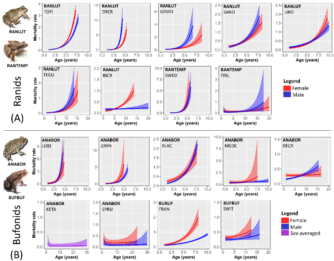
Fig. 2. Mortality curves for males (blue) and females (red) of 18 ranid (A) and bufonid (B) populations from North America and Europe. Two ranid species, Rana luteiventris (RANLUT) and Rana temporaria (RANTEMP), and two bufonid species, Anaxyrus boreas (ANABOR) and Bufo bufo (BUFBUF), were considered. The parameters a_0 and a_1 extracted from the Siler model did not converge for one population of R. luteiventris (POCR); furthermore, for one population of A. boreas (LOTA), credible intervals of mortality rate early in life were very large. Senescence patterns are thus not displayed for these two populations but parameter estimates are available in Supplementary material (Tables S16 and S23) . Age presented on the x -axis of mortality curves corresponds to the age from onset of adulthood.
