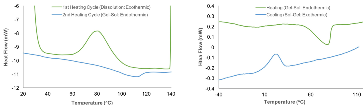
Figure 5. DSC of a) 12 wt% MCC in [P_{4441}][OAc]:GVL (70:30 w/w) from frozen to observe the sign of the initial exothermic ‘dissolution’ enthalpy and b) 20 wt% MCC in [P_{4441}][OAc]:DMSO (80:20 w/w) to observe the reversible endothermic gel-sol transition, after exothermic dissolution and cooling.
