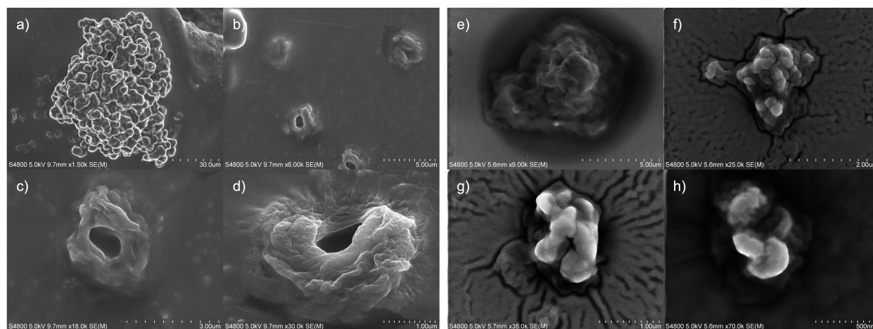
Figure 11. SEM analysis of cellulose microparticles after regeneration from [P_{4441}][OAc]:GVL (a–d) and washing away of residual [P_{4441}][OAc] using acetone and ultrasonication (e–f): a) microparticle cluster, b–d) separated microparticles retained on the support after flushing with nitrogen, e–h) aggregated and fully regenerated microparticles of different sizes after washing away the [P_{4441}][OAc] .
