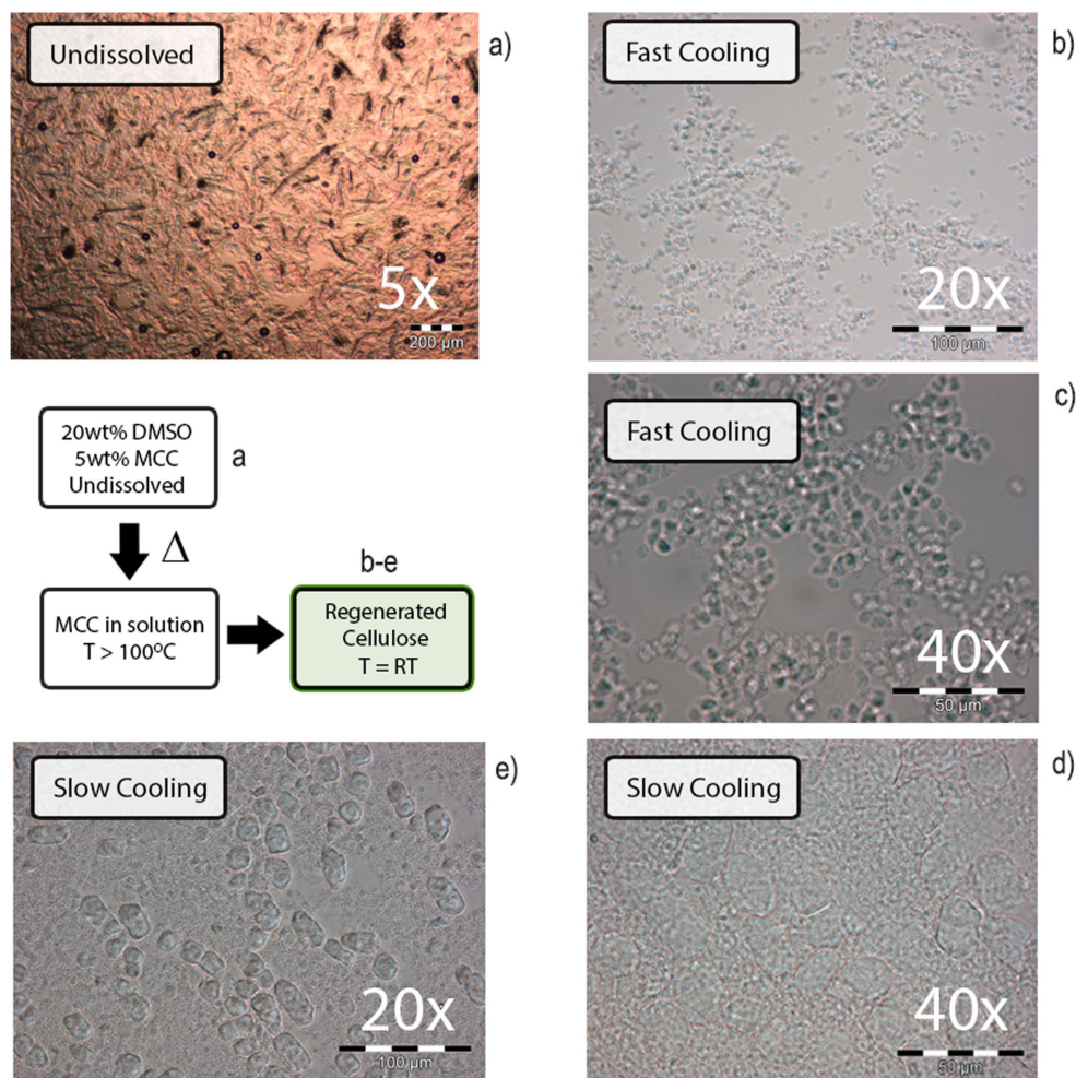
Figure 10. Variation in particle size upon regeneration of 5 wt% MCC from [\text{P}_{4441}][\text{OAc}]:\text{DMSO} (80:20 w/w) at different cooling rates; slow cooling by letting sit on the bench and fast cooling by cooling in an ice bath.
