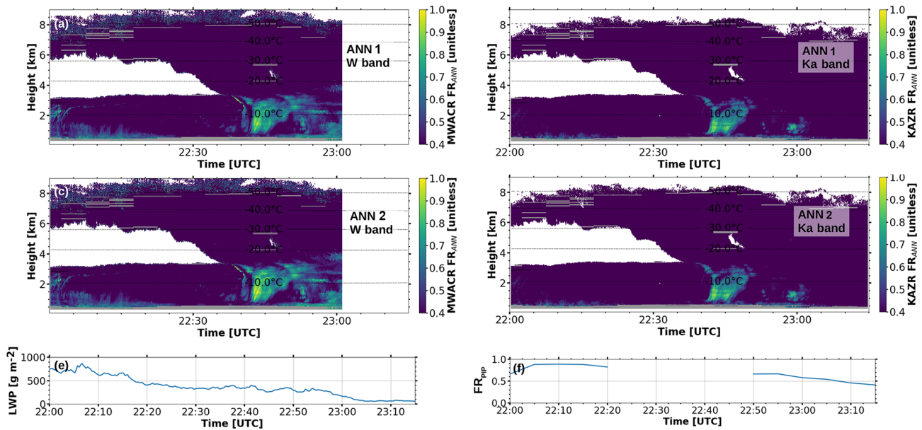
Figure 4. Riming during the focus case on 21 February 2014 as predicted by (a, b) ANN 1 trained on MWACR and KAZR data, respectively (Ze, MDV, SEW, and skewness), and (c, d) ANN 2 trained on MWACR and KAZR data, respectively (Ze, SEW, and skewness). (e) Liquid water path obtained from microwave radiometer measurements. (f) FR_{RIP} measured during the event. Pixels with EDR above the threshold of 10^{-3} \text{ m}^2 \text{ s}^{-3} are masked in gray in panels (a)–(d).
