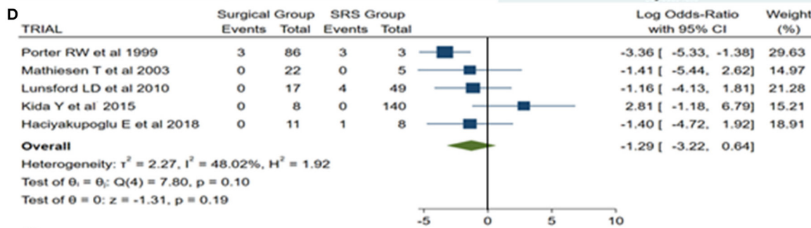
Random-effects REML model
