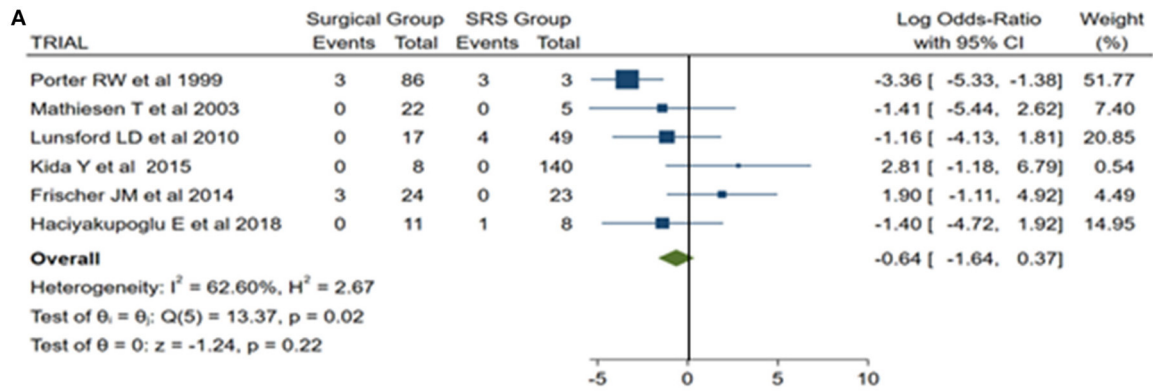
Fixed-effects Mantel-Haenszel model
