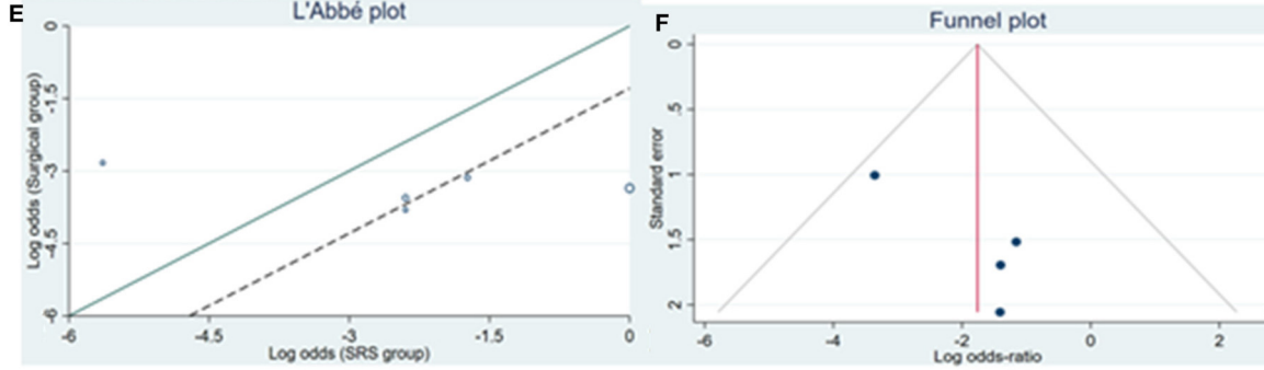
Random-effects REML model
