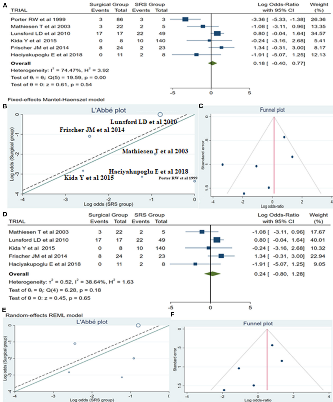
FIGURE 3 | Rebleeding (ReBl): (A) OR forest plot ReBl: Results demonstrate no statistically significant difference between the two groups [decimal logarithm of odd ratio—log OR 0.18, CI 95% -0.40 to 0.77, and p = 0.54 ]; (B) L'Abbé plot and analysis of heterogeneity ( p < 0.1 and I^2 = 74.47\% ); (C) Funnel plots for publication bias on the available evidence relevant to BSCMs management; (D) OR forest plot ReBl without “Porter RW” (11) article: Results demonstrate no statistically significant difference between the two groups (log OR 0.24, CI 95% -0.80 to 1.28, and p = 0.65 ); (E,F) L'Abbé and funnel plots demonstrated very low heterogeneity ( p = 0.18 and I^2 = 38.64\% ) and no publication bias of the ReBl in groups of patients with BSCMs, respectively. SRS, Radiosurgical group; I^2 shows the percentage of total variation across studies that is due to heterogeneity rather than chance; CI, confidence interval.
