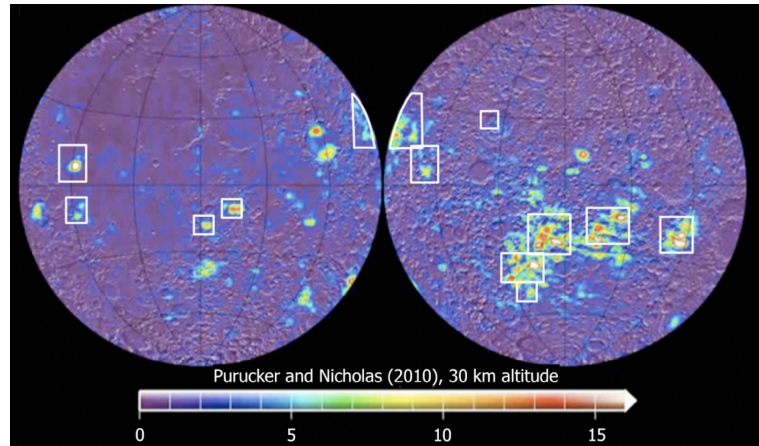
Figure 1: Magnetic field strengths across the lunar surface. White boxes are locations of identified swirls.
