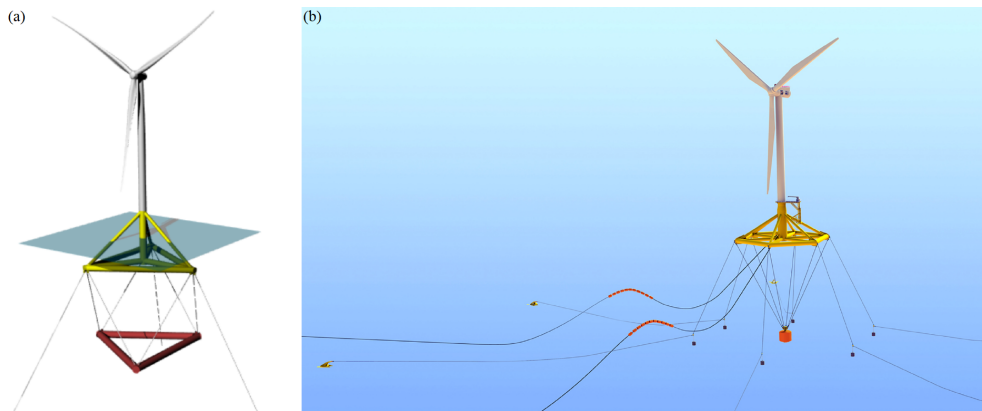
Figure 6. Pendulum-stabilized innovative floating platform concepts. (a) Stiesdal's TetraSpar (Borg et al., 2020). (b) Saipem's Hexafloat (Ribout, 2019).
