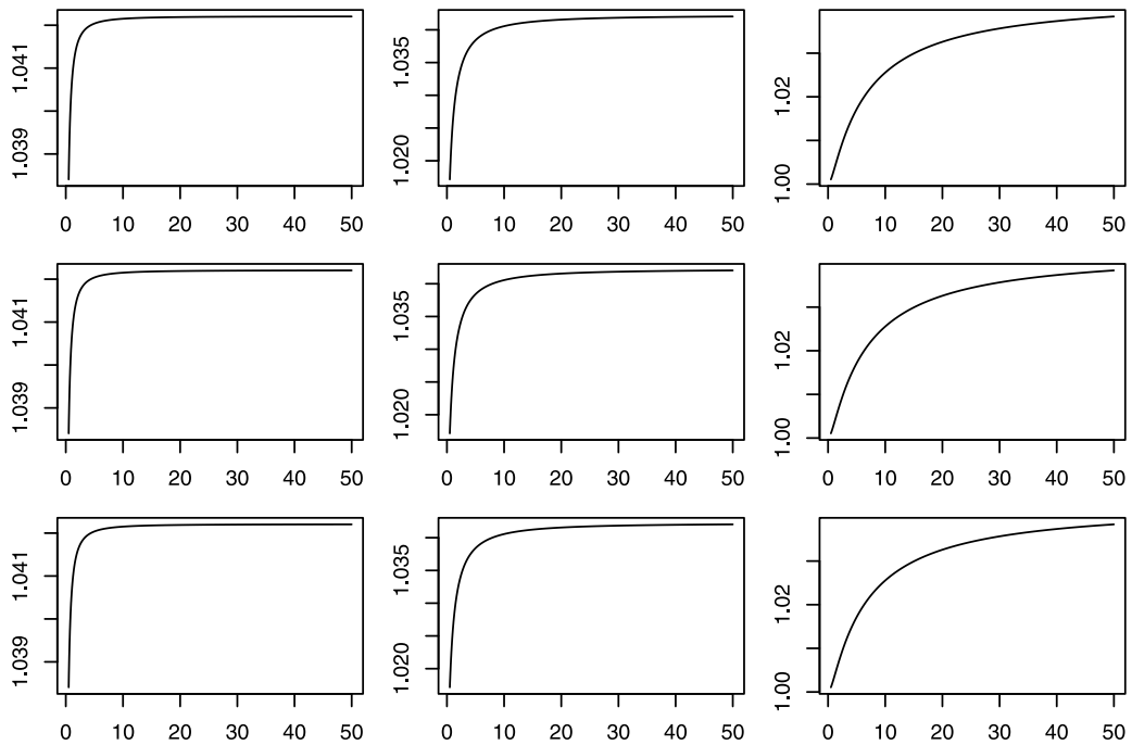
Fig. 2. Plot of the ratio \frac{\hat{f}_{X_1}(x;\theta)}{f_{X_1}(x;\theta)} for different values of a and b , with \lambda fixed at 2. In each row, b takes a value from \{0.1, 1, 10\} ; in each column, a takes a value from \{0.1, 1, 10\} . The x -axis represents the value of x .
