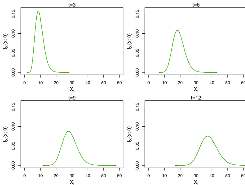
Fig. 7. Density plots of f_{X_t}(x; \theta) (black), \hat{f}_{X_t}(x; \theta) (red) and \bar{f}_{X_t}(x; \theta) (green), when t increases.
