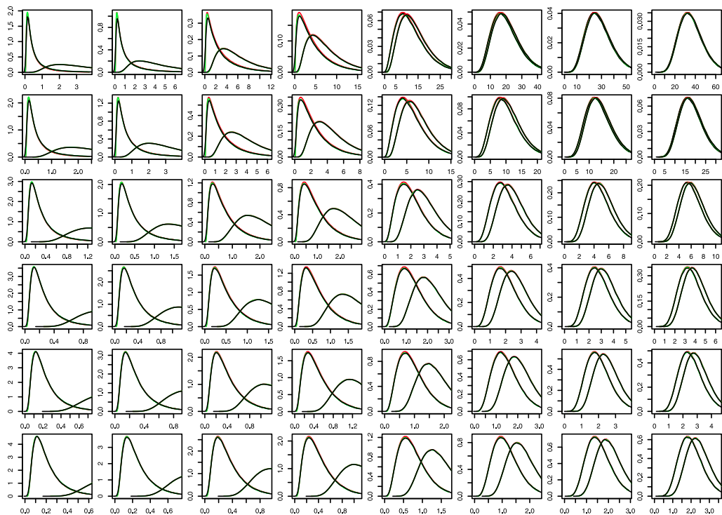
Fig. 12. Density plots of f_{X_1}(x; \theta) (black), \hat{f}_{X_1}(x; \theta) (red) and \tilde{f}_{X_1}(x; \theta) (green). In each row, \lambda takes in turn a value from \{-0.75, -0.25, 0.5, 1, 3, 5, 7, 9\} . In each column, a takes in turn a value from \{0.5, 1, 3, 5, 7, 9\} . In each panel, b takes values 0.5 and 9.
