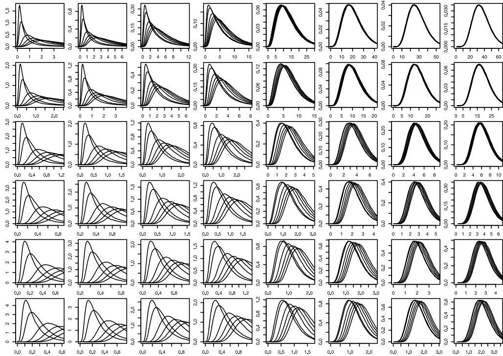
Fig. 11. Density plots of GIG(\lambda, a, b) . In each row, \lambda takes in turn a value from \{-0.75, -0.25, 0.5, 1, 3, 5, 7, 9\} . In each column, a takes in turn a value from \{0.5, 1, 3, 5, 7, 9\} . In each panel, b takes in turn a value from \{0.5, 1, 3, 5, 7, 9\} .
