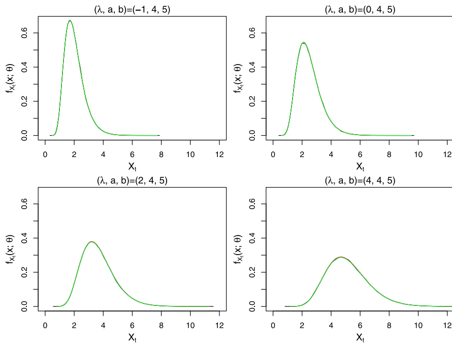
Fig. 6. Density plots of f_{X_t}(x; \theta) (black), \hat{f}_{X_t}(x; \theta) (red) and \bar{f}_{X_t}(x; \theta) (green), when \lambda increases.
