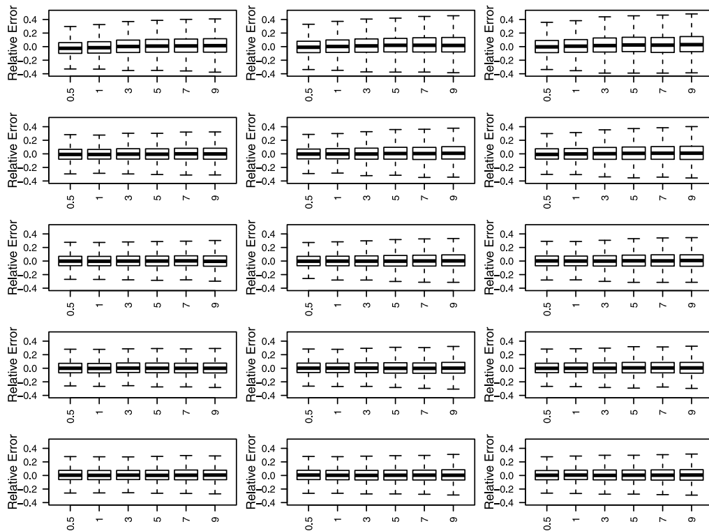
Fig. 8. Box plots of the relative errors of the ML estimates \hat{a} , with the value of b being known. In each column, \lambda takes in turn a value from \{1, 3, 5, 7, 9\} . In each row, b takes in turn a value from \{1, 3, 5\} . In each panel, a takes in turn a value from \{0.5, 1, 3, 5, 7, 9\} .
