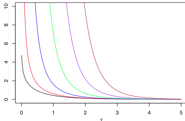
Fig. 1. Plot of the modified Bessel functions of the second kind: K_0(v) (black), K_1(v) (red), K_2(v) (blue), K_3(v) (green), K_4(v) (purple), K_5(v) (brown).
