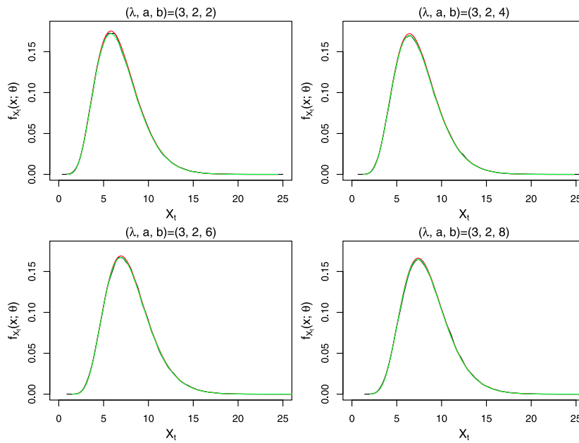
Fig. 4. Density plots of f_{X_t}(x; \theta) (black), \hat{f}_{X_t}(x; \theta) (red) and \bar{f}_{X_t}(x; \theta) (green), when b increases.
