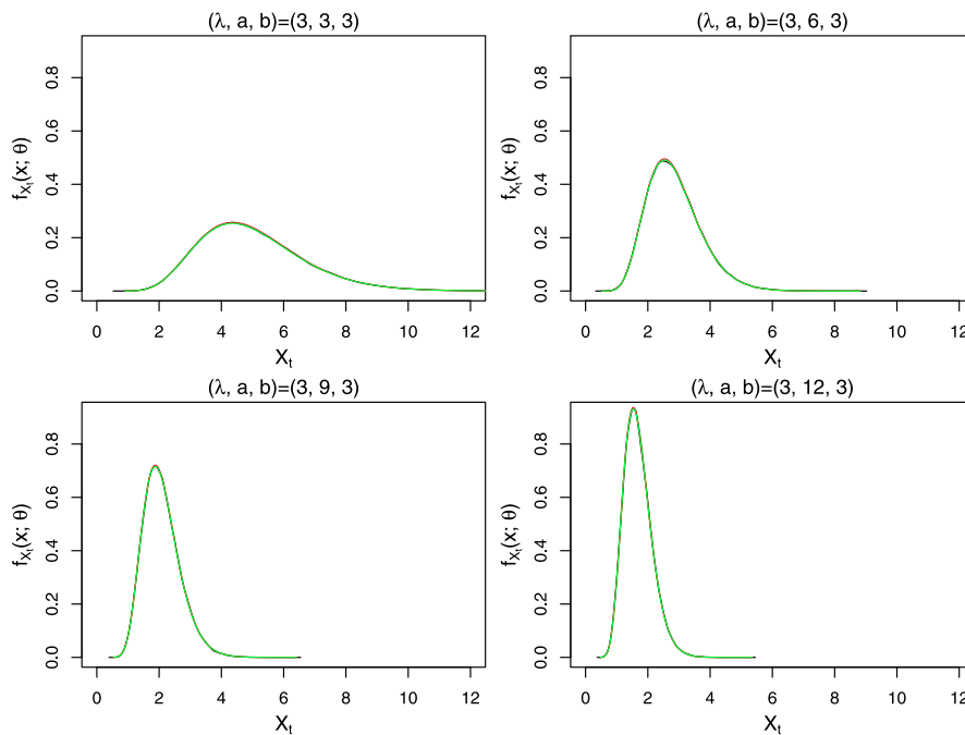
Fig. 5. Density plots of f_{X_t}(x; \theta) (black), \hat{f}_{X_t}(x; \theta) (red) and \bar{f}_{X_t}(x; \theta) (green), when a increases.
