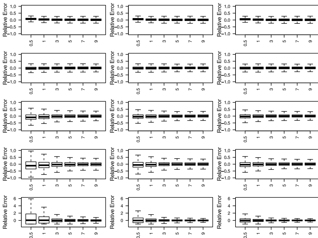
Fig. 9. Box plots of the relative errors of the ML estimates \hat{b} , with the value of \lambda being known. In each column, \lambda takes in turn a value from \{-0.75, -0.25, 0.5, 1, 3\} . In each row, a takes in turn a value from \{1, 3, 5\} . In each panel, b takes in turn a value from \{0.5, 1, 3, 5, 7, 9\} .
