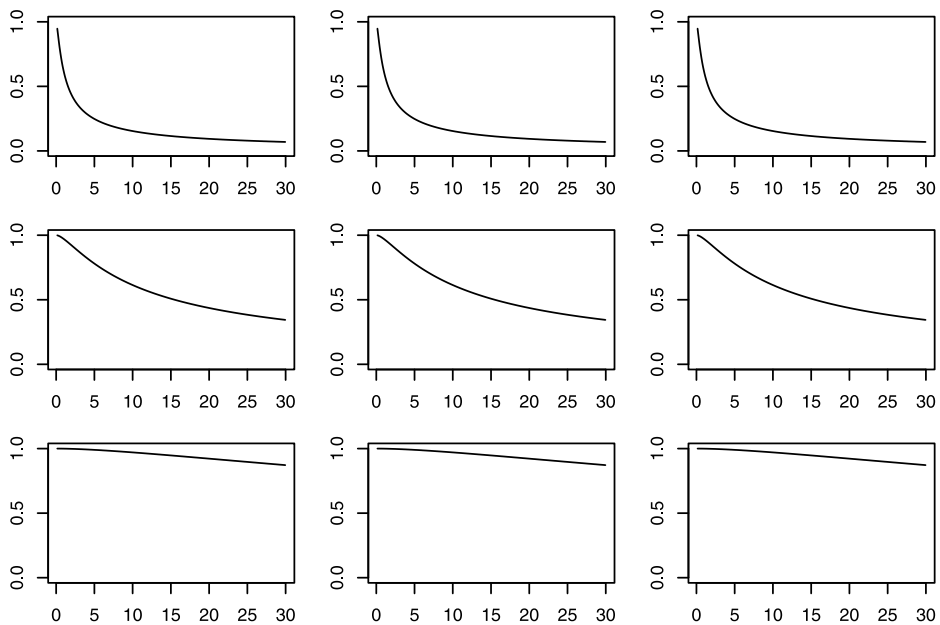
Fig. 3. Plot of the ratio \frac{\hat{f}_{X_1}(x;\theta)}{f_{X_1}(x;\theta)} for different values of a and b , with \lambda fixed at -0.75 .
