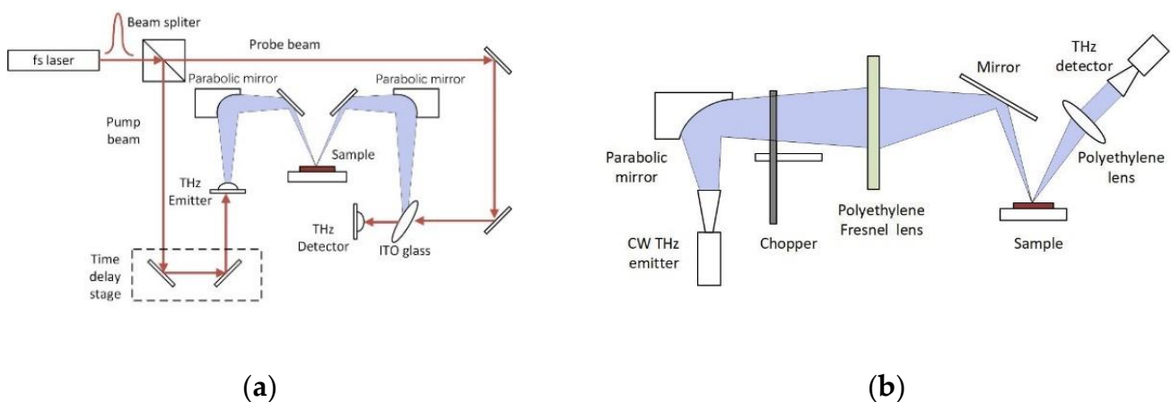
Figure 1. (a) Schematic diagram of a pulsed TD THz imaging system. (b) Schematic diagram of a CW THz imaging system.
