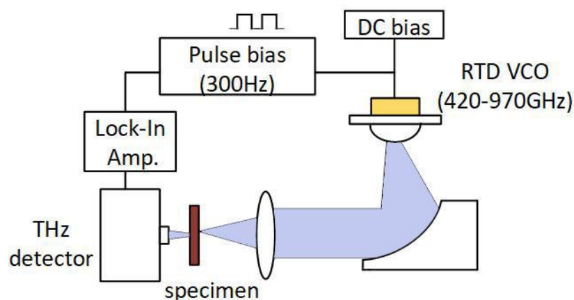
Figure 8. Schematic diagram of wide bandwidth RTD spectroscopy system. Adapted with permission from Ref. [69].
