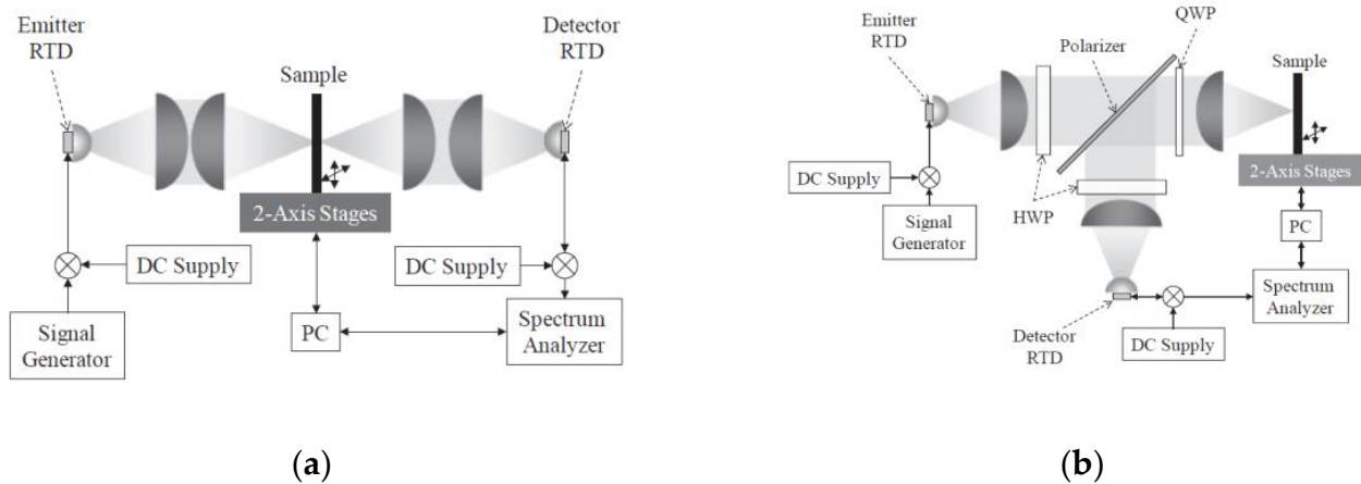
Figure 6. (a) THz transmission imaging system using RTD transceiver. (b) THz reflection imaging system using RTD transceiver. Reprinted with permission from Ref. [60].
