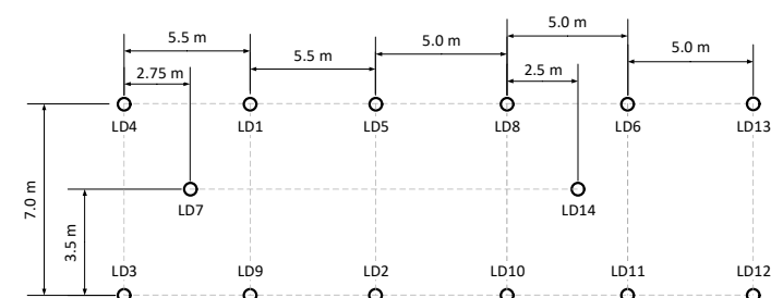
Figure 2 Pile layout plan
