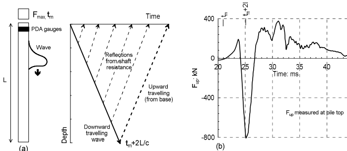
Figure 4 Schematic of stress waves travelling in a pile
