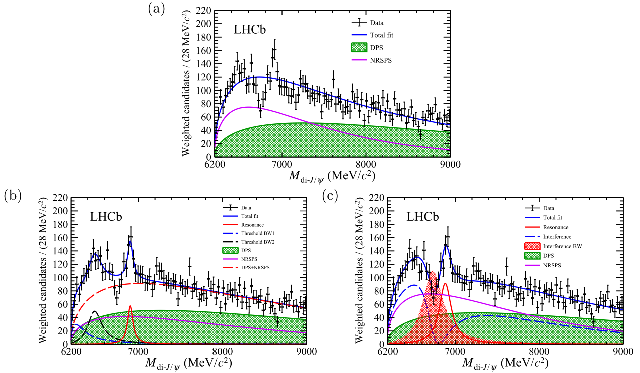
Fig. 3. Invariant mass spectra of weighted di- J/\psi candidates with p_{\text{T}}^{\text{di-}J/\psi} > 5.2 GeV/ c and overlaid projections of the p_{\text{T}}^{\text{di-}J/\psi} -threshold fit using (a) the NRSPS plus DPS model, (b) model I, and (c) model II.
