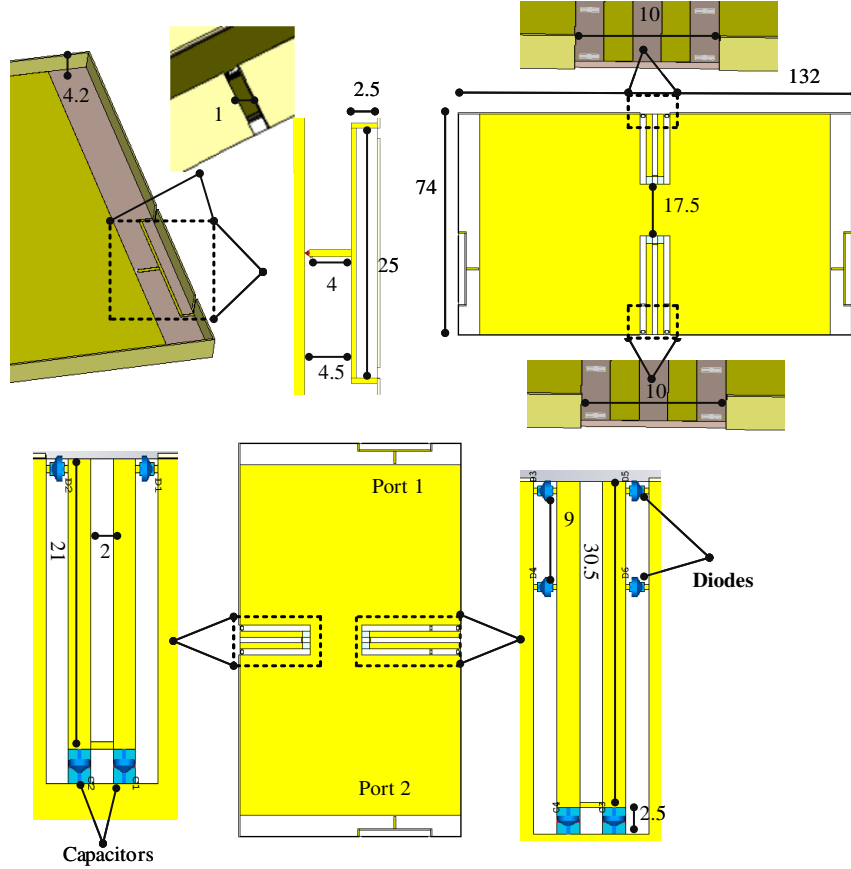
Figure 1. Geometry of the proposed dual band 2 \times 2 MIMO-based rim antenna, with all the units in millimeters (mm) and the structure is displayed and explained using multiple views. [reproduced courtesy of The Electromagnetics Academy]
