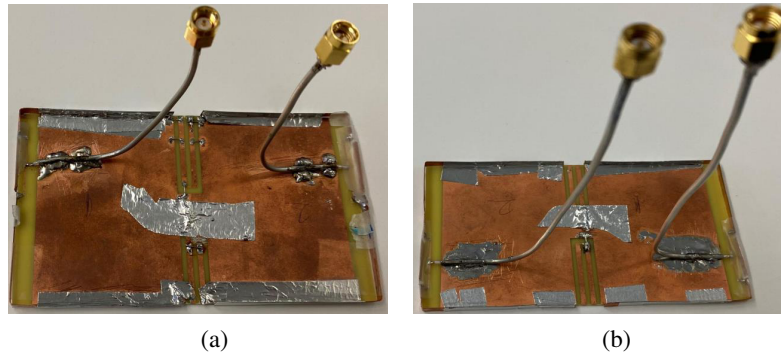
Figure 5. Prototype of (a) DGS ON configuration, (b) DGS OFF configuration of the proposed rim antenna design. [Figure 4 & 5 reproduced courtesy of The Electromagnetics Academy]
