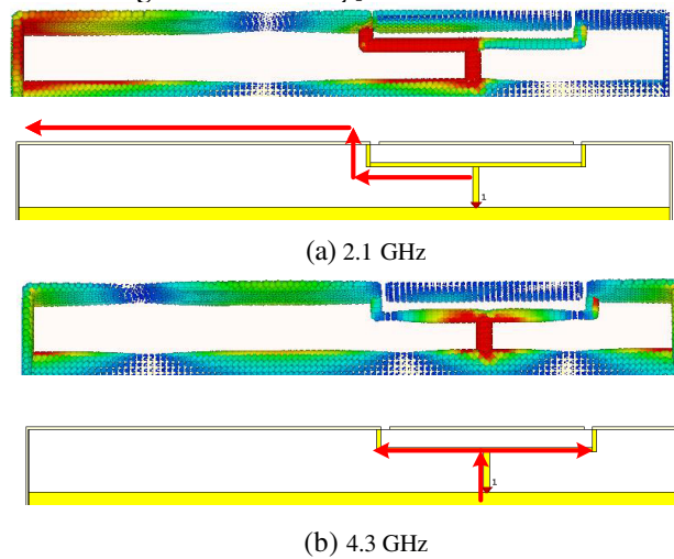
Figure 3. Simulated surface current plots at 2.1 GHz and 4.3 GHz. [reproduced courtesy of The Electromagnetics Academy]
