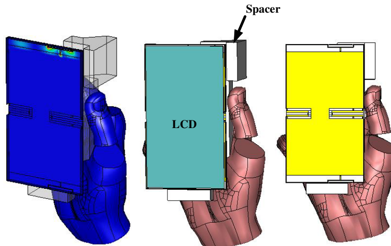
Figure 9. An illustration of the effect of hand and LCD on the proposed rim antenna design. [reproduced courtesy of The Electromagnetics Academy]
