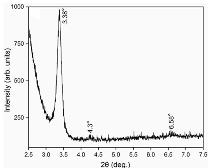
Fig. 2. Low-angle XRD diffraction patterns of TiN/NbN multilayer coating.
