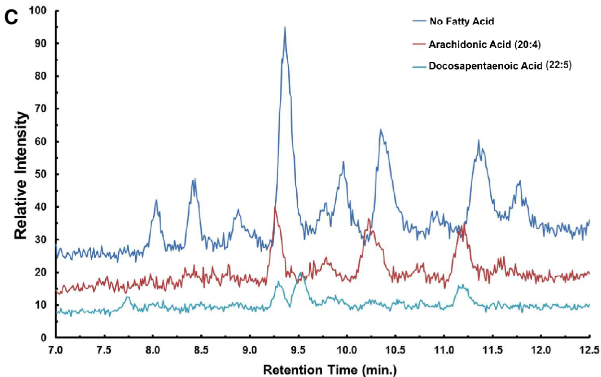
Figure 6: Ultra performance liquid chromatography (UPLC) and mass spectrometry of A. baumannii phospholipid species. Bacteria were grown in G-56 (pH 7.4) at 37°C with or without various fatty acids. Phospholipids were dissolved in 50:50 mobile phase A:B and injected into a Waters UPLC with reversed-phase C8 column. Detection was quadropole mass spectrometry. The changes in retention time (and mass spectra) are consistent with incorporation of the exogenous fatty acids into the phospholipids of A. baumannii during growth in 37°C. In Figure A, chromatograms are shown for bacteria grown with 18:3 , 20:5, and 22:6; figure B represents chromatograms for bacteria grown in the presence of fatty acids 18:2, 18:3 , and 20:3; figure C shows chromatograms for A. baumannii grown with 20:4 and 22:5. Predicted structures are provided in A, reflecting the eluted phospholipid species.
