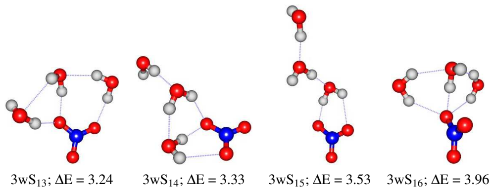
Figure S2: Structural motifs with energies larger than 3 kcal mol -1 of the global minimum on the potential energy surface for [NO 3 (H 2 O) 3 ] - . Dotted lines correspond to intermolecular contacts, those for which AIM predicts bonding paths. Data taken from the PBE0PBE1/Def2-PVTZ optimized geometries
