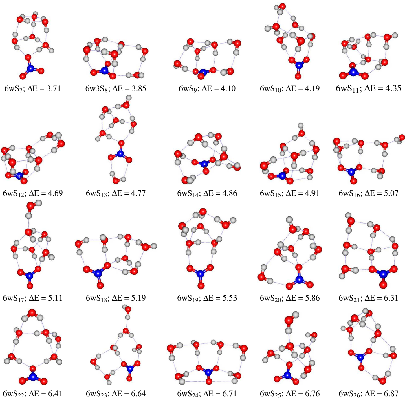
Figure S5: Structural motifs with energies larger than 3 \text{ kcal mol}^{-1} of the global minimum on the potential energy surface for [\text{NO}_3(\text{H}_2\text{O})_6]^- . Dotted lines correspond to intermolecular contacts, those for which AIM predicts bonding paths. Data taken from the PBE0PBE1/Def2-PVTZ optimized geometries
