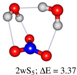
Figure S1: Structural motifs with energies larger than 3 kcal mol -1 of the global minimum on the potential energy surface for [NO 3 (H 2 O) 2 ] - . Dotted lines correspond to intermolecular contacts, those for which AIM predicts bonding paths. Data taken from the PBE0PBE1/Def2-PVTZ optimized geometries
