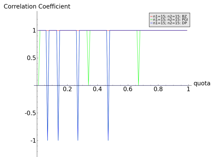
Fig. 4 Similarity indices for Case-II.
