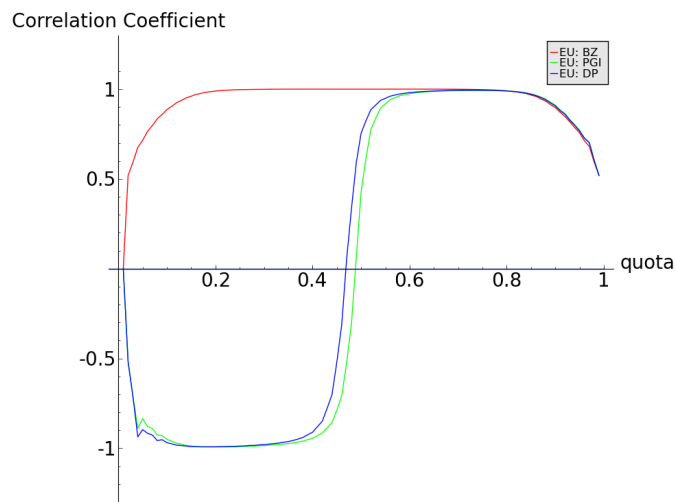
Fig. 13 Similarity indices for EU weights.
