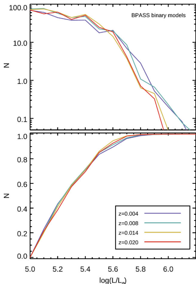
Figure 9. Top: Predictions of the luminosity function of cool supergiants from BPASS binary population synthesis for the metallicity range Z = 0.004 – 0.020 . Bottom: The same result but shown as a cumulative luminosity distribution.
