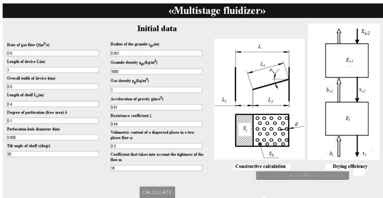
Fig. 1 The main page of the Multistage fluidizer® software [21]
