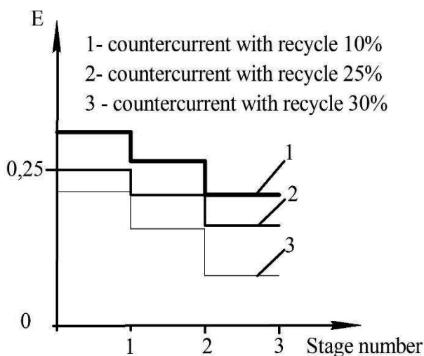
Fig. 6 An influence of the drying agent recirculation method on the drying efficiency (stage number - in the direction of movement of disperse material)
