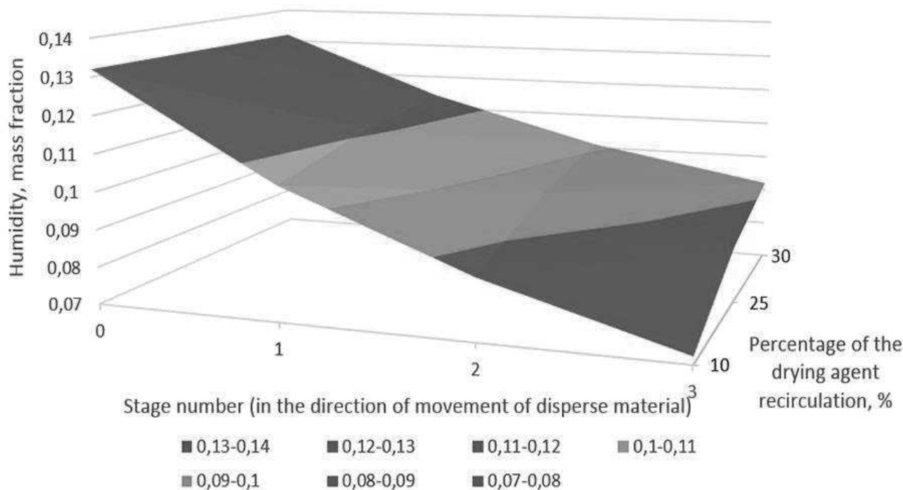
Fig. 2 An influence of the drying agent recirculation method on the change of the moisture content in the disperse material
