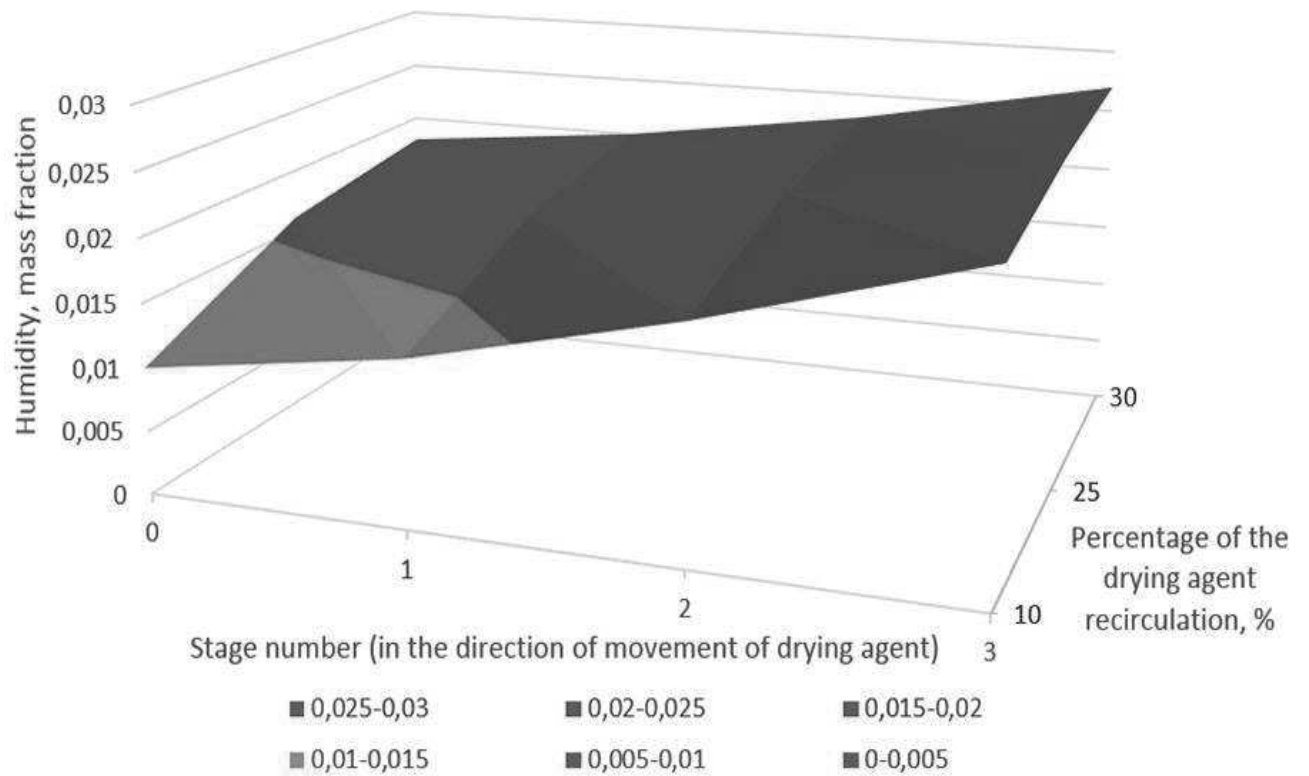
Fig. 3 An influence of the drying agent recirculation method on the change of the moisture content in the drying agent
