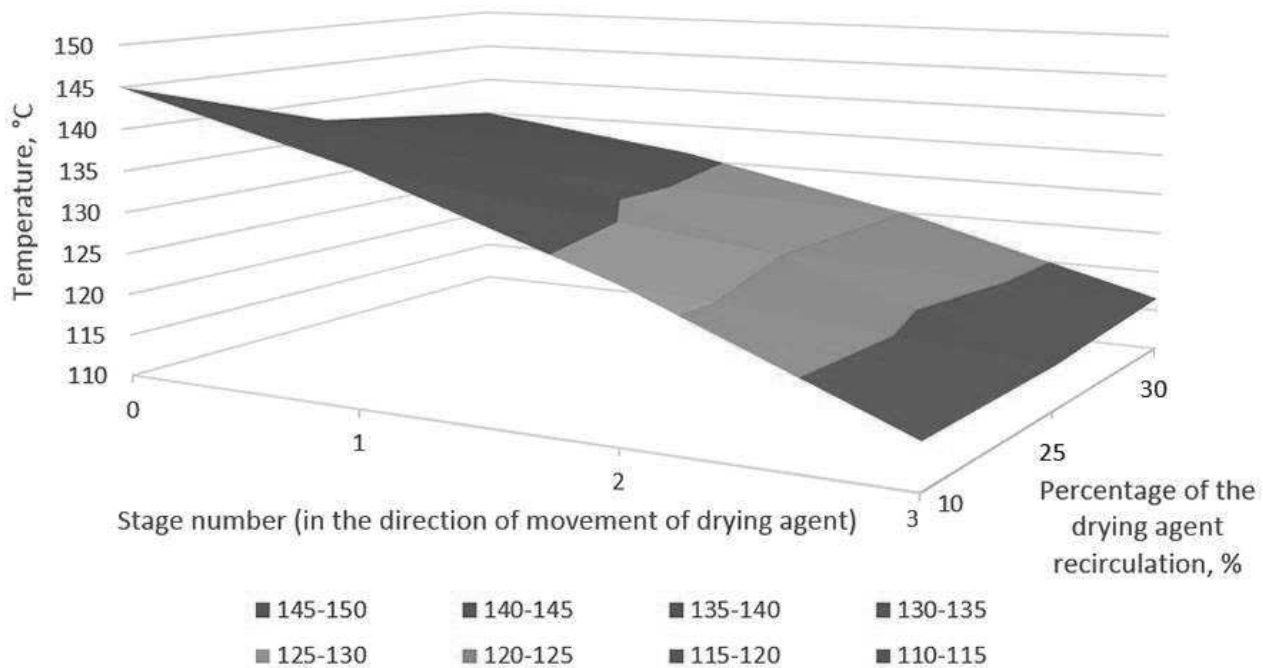
Fig. 5 An influence of the drying agent recirculation method on the temperature change of the drying agent
