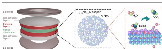
Figure 1. Structure and performance characteristics of proton exchange membrane fuel cell (PEMFC) gas sensor. Left: schematic illustration of PEMFC sensor. Middle: microstructure of sensing layer of working electrode. Right: gas sensing at the working electrode (take formaldehyde detection as an example).
