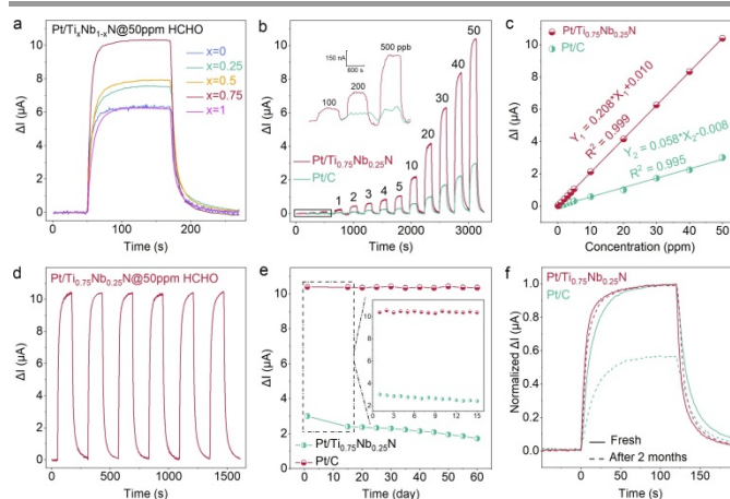
Figure 3. a) The response transients of Pt/Ti x Nb 1-x N sensor to 50 ppm formaldehyde. b) Real-time responses and c) formaldehyde concentration dependent response value of Pt/Ti x Nb 1-x N and Pt/C sensor to 0.1-50 ppm formaldehyde. d) The 6-cycle dynamic sensor response verifies the repeatability of the Pt/Ti 0.75 Nb 0.25 N sensor to 50ppm formaldehyde. e) Comparison of response attenuation of Pt/Ti 0.75 Nb 0.25 N and Pt/C-based sensor in detecting 50ppm formaldehyde within two months. f) Normalized real-time responses of Pt/Ti 0.75 Nb 0.25 N and Pt/C-based sensor to 50 ppm formaldehyde at different aging states.
