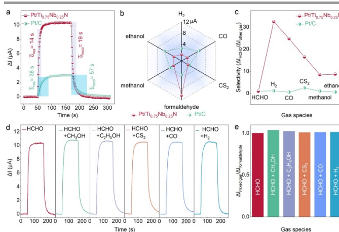
Figure 4. a) Real time response transient of Pt/Ti 0.75 Nb 0.25 N and Pt/C sensor to 50 ppm formaldehyde (HCHO). b) Selectivity and c) selectivity improvements for Pt/Ti 0.75 Nb 0.25 N and Pt/C sensor toward various analyte gases. d) Sensor response of Pt/Ti 0.75 Nb 0.25 N to a transient of 50 ppm formaldehyde followed by five transients of mixed gases of 50 ppm formaldehyde and 50 ppm methanol (CH 3 OH), 50 ppm ethanol (C 2 H 5 OH), 50 ppm carbon disulfide (CS 2 ), 50 ppm carbon monoxide (CO) and 50 ppm hydrogen (H 2 ), respectively. e) The response of the sensor fluctuates only slightly during exposure to different gas mixtures.
