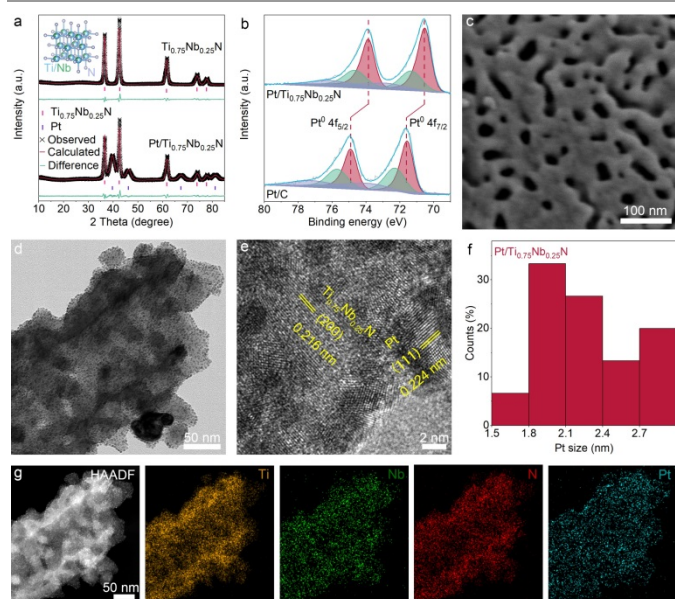
Figure 2. a) The Rietveld fitted powder X-ray diffraction pattern of Ti 0.75 Nb 0.25 N and Pt/Ti 0.75 Nb 0.25 N. b) X-ray photoelectron spectroscopy spectra of Pt/Ti 0.75 Nb 0.25 N and Pt/C (Johnson Matthey) in the Pt 4f region. c) SEM images of Ti 0.75 Nb 0.25 N. d) TEM images of Pt/Ti 0.75 Nb 0.25 N and e) HRTEM image of Pt/Ti 0.75 Nb 0.25 N. f) Pt size distribution of Pt/Ti 0.75 Nb 0.25 N. g) HAADF-STEM image and corresponding elemental mapping of EDX mapping images of Ti, Nb, N and Pt.
