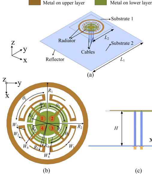
Fig. 1. Configuration of the proposed antenna. (a) 3D view. (b) top view. (c) side view. Dimensions are L_1 = 140 , L_2 = 60 , W_1 = 3.8 , W_2 = 0.5 , W_3 = 1 , W_4 = 0.5 , W_5 = 2.4 , W_6 = 1 , R_1 = 25 , R_2 = 22.2 , R_3 = 17.3 , R_4 = 14 , R_5 = 10.5 , R_6 = 9 , R_7 = 7.5 , H = 34 , \theta_1 = 80^\circ , \theta_2 = 78^\circ , and \theta_3 = 70^\circ (unit: millimeter).
