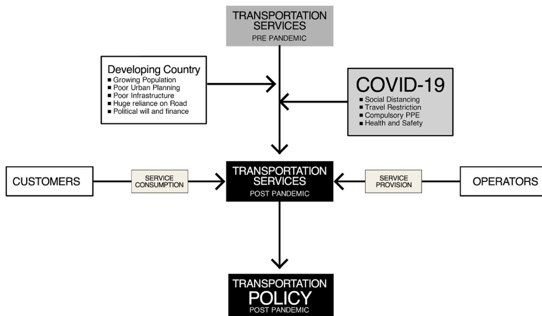
Fig. 2. Conceptual framework.
