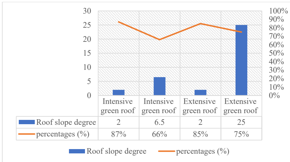
Figure 7: Performance of Intensive and Extensive green roof based on roof slope
