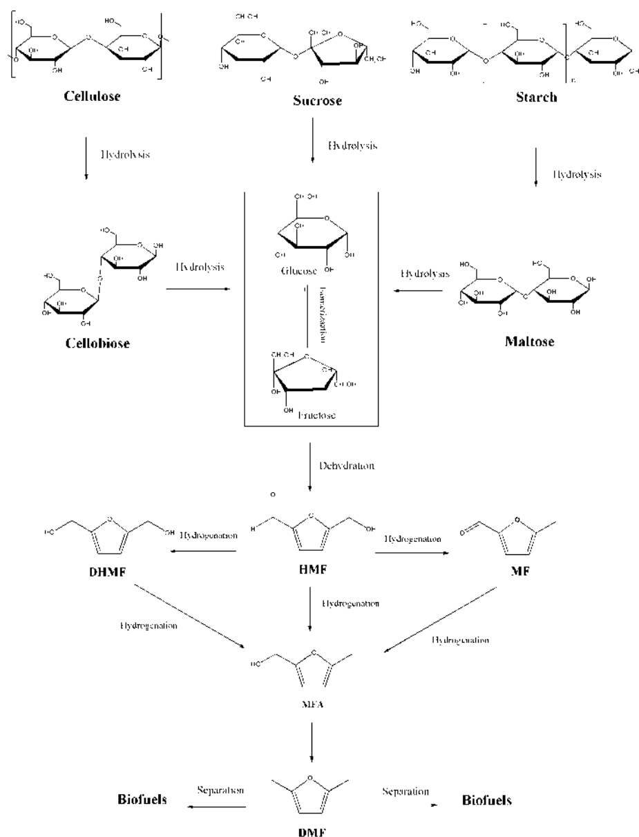
Scheme 1. Integrated reaction pathway for the transformation of biomass-derived carbohydrates into DMF. Adapted from [40].
