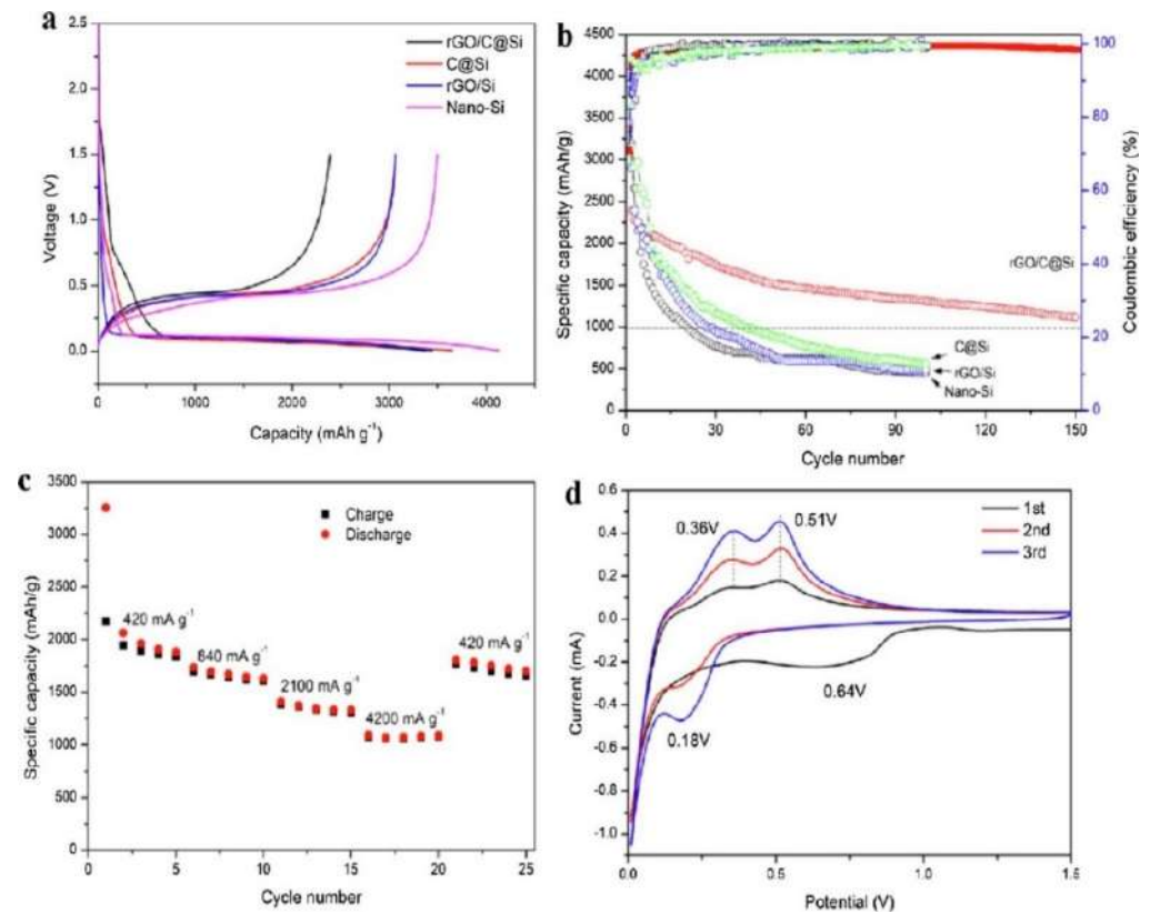
Figure 9. Electrochemical evaluations of fabricated anodes. (a) Initial charge/discharge of nano-Si, C@Si, rGO/Si and rGO/C@Si nanocomposites at a current density of 100 mA g -1 , (b) consistent current charge/discharge of nanocomposites and (c,d) rate performance and current/voltage profile of GO/C@Si anode [158].
