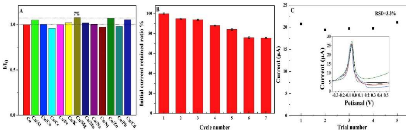
Figure 8. (A) Selectivity, (B) repeatability and (C) reproducibility of chitosan/GO/ion imprinting polymer (CS/GO/IIP) as an electrochemical sensor for Cu (II) detection ( 50 \mu\text{mol/L} ) [143].
