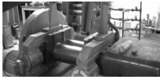
b) Types of open roll mills used for mixing
