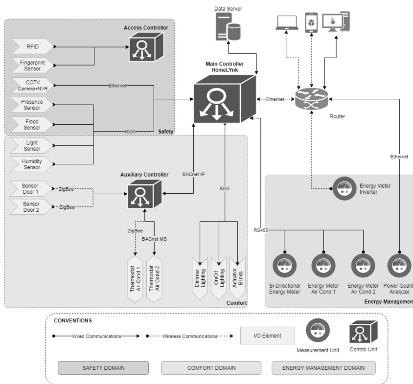
Figure 5. System Model: Class diagram grouped by domain. Source: The authors
