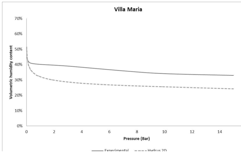
Figure 2. Experimental and Hydrus 2D humidity retention curves for Villa María farm at 0 to 10 cm depth.
