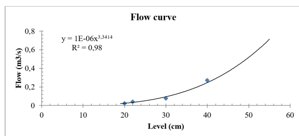
Figure 3. Flow curve example.
