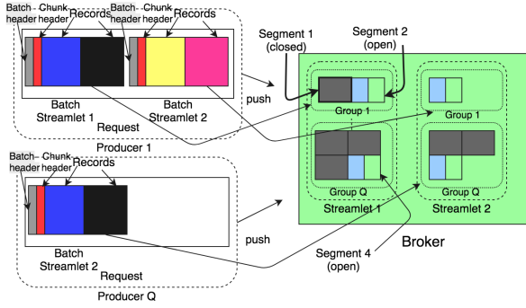
Fig. 3: Representation of records, chunks, segments, groups, and streamlets illustrates how producers aggregate records into requests and push them to brokers. Each request contains multiple chunks (chunk and request size are configurable). We exemplify a stream composed of two streamlets. A streamlet holds up to Q active groups (fixed-size sub-partitions) for new appends. A producer writes to the streamlet's active group corresponding to the entry calculated as producer identifier modulo Q .
