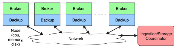
Fig. 1: The architecture of a stream storage system: the coordinator manages storage nodes on which live broker and backup processes. Clients mainly interact with brokers since they control the active partition replicas. Backups handle the passive partition replicas and are later involved in fault tolerance recovery.
