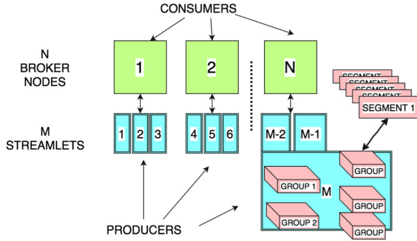
Fig. 4: Semantic partitioning of streams with streamlets. A stream is composed of a set of streamlets (partitions). Each streamlet is composed of an unbounded set of fixed-size sub-partitions called groups of segments.
