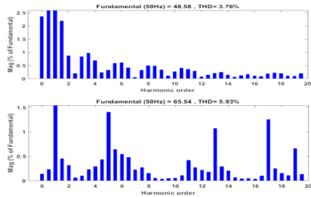
Figure 7. THD of source current with PI controller
