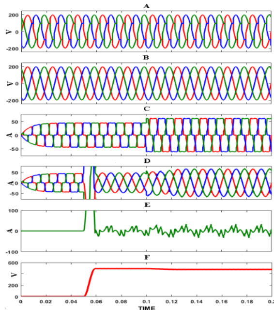
Figure 8. Shunt HAPF response with ANN controller
