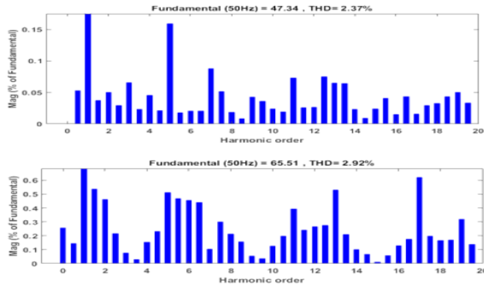
Figure 9. THD of source current with ANN controller
