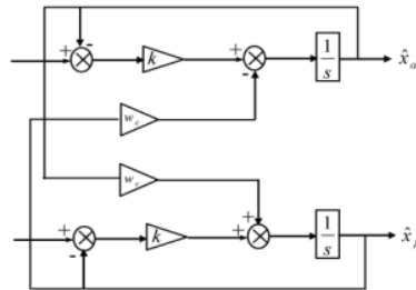
Figure 1. Self-tuning filter
