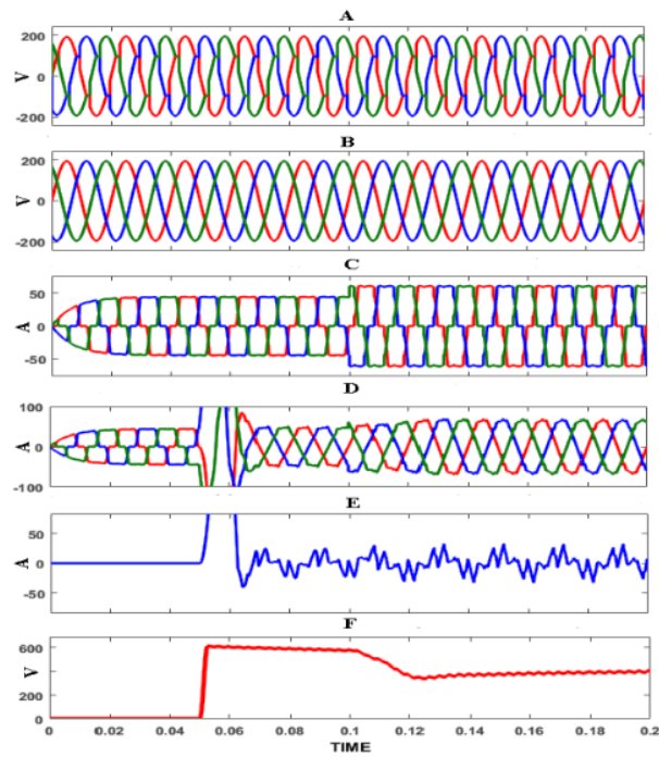
Figure 6. Shunt HAPF responses with PI controller
