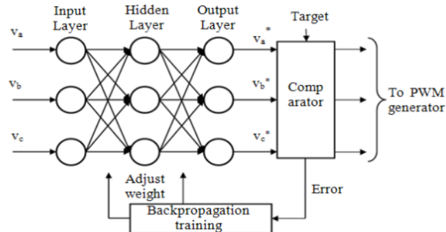
Figure 4. The block diagram of ANN controller
