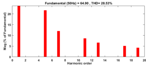
Figure 5. THD of source current without a filter
