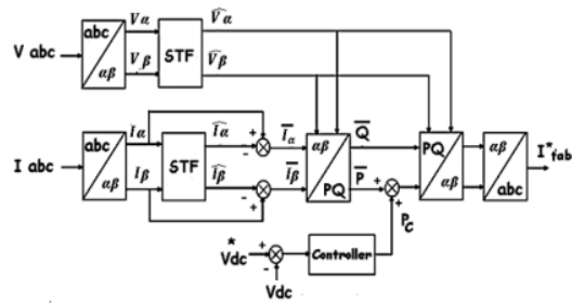
Figure 2. Control algorithm of HPF
